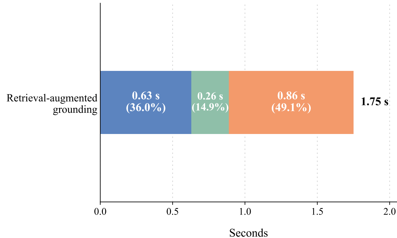
(b) Runtime composition of retrieval-augmented grounding
