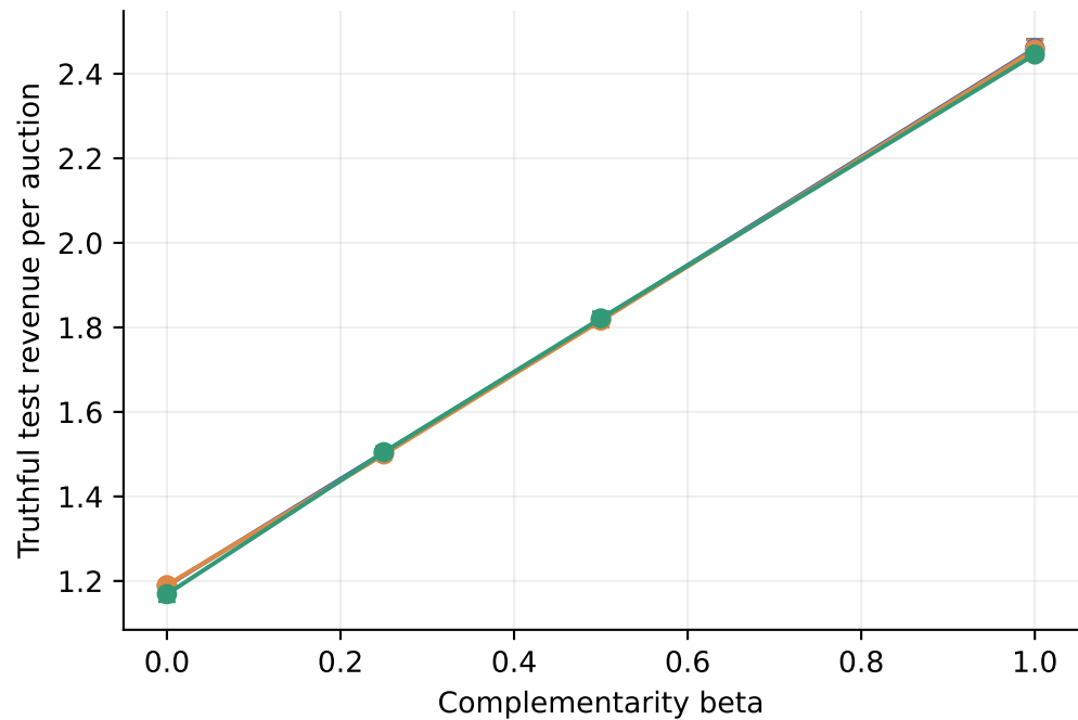
E3 complementarity strength — five-seed mean \pm SD; n=2 , m=3
