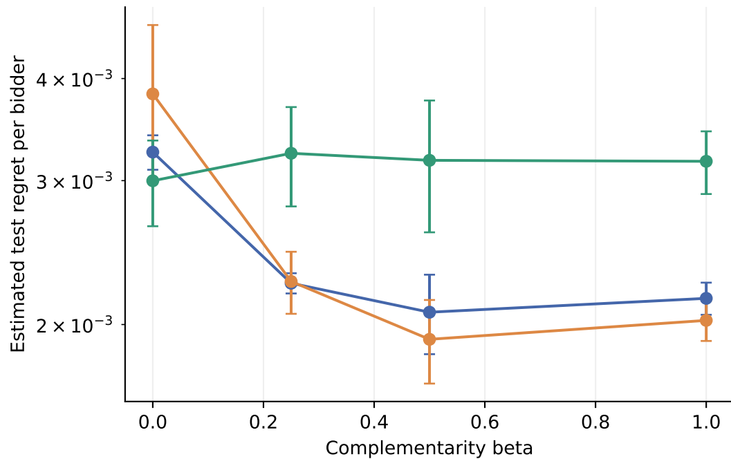
E3 complementarity strength — five-seed mean \pm SD; n=2 , m=3
