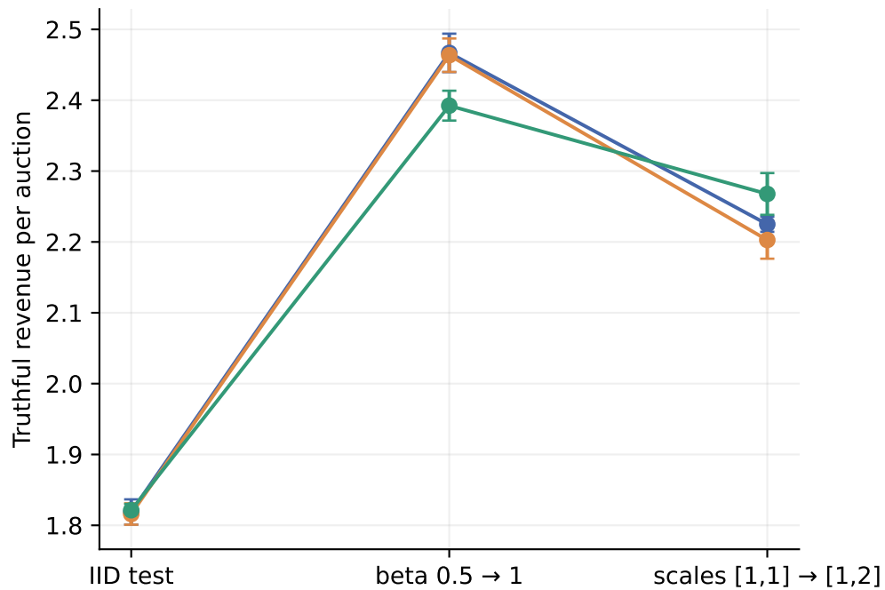
E5 held-out distribution shifts — no retraining; mean \pm SD
