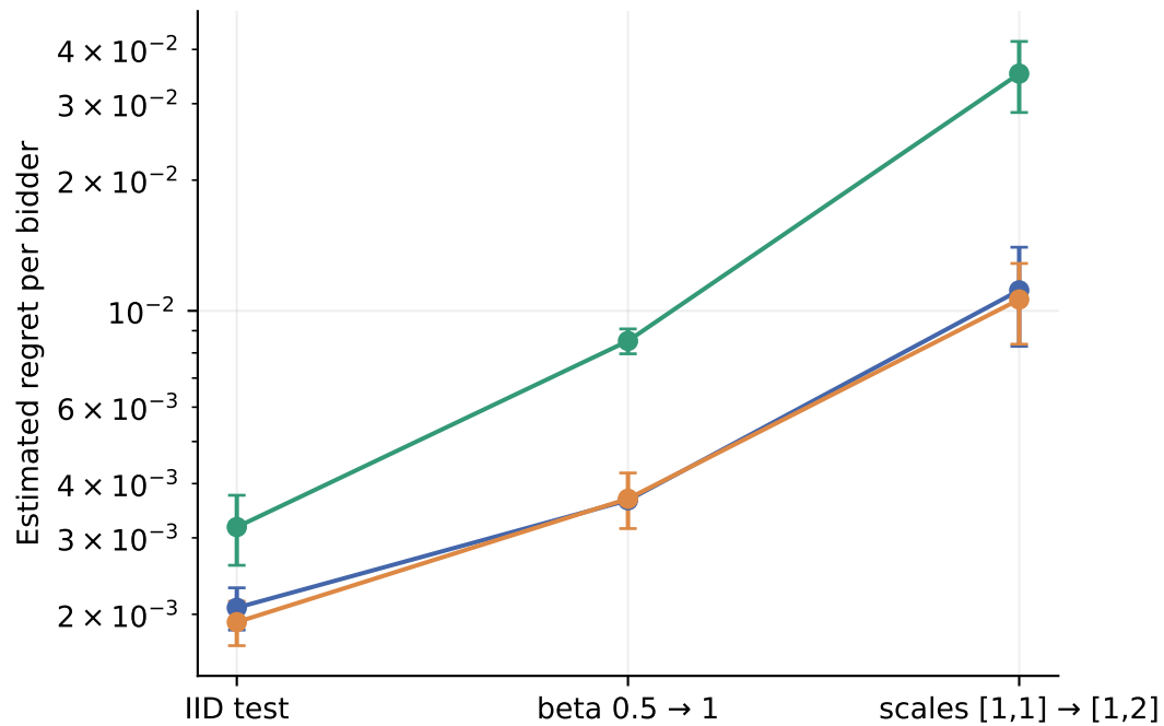
E5 held-out distribution shifts — no retraining; mean \pm SD
