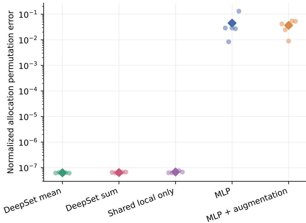
E5 and ablations — permutation error: five seeds (circles), mean (diamonds)
