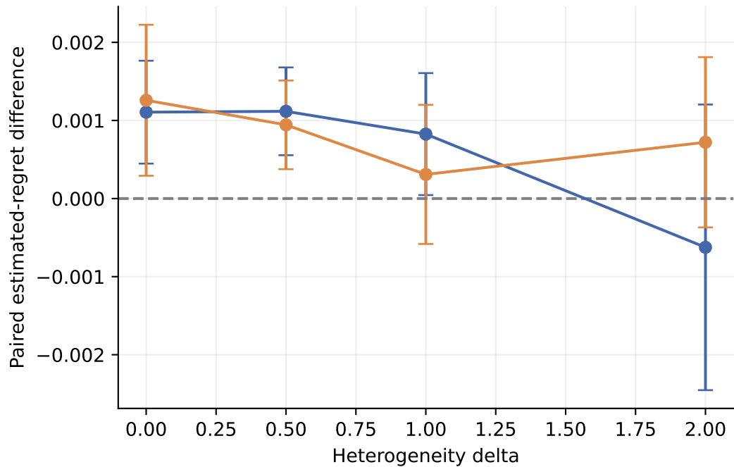
E4 paired differences — descriptive 95% t intervals, five seeds
