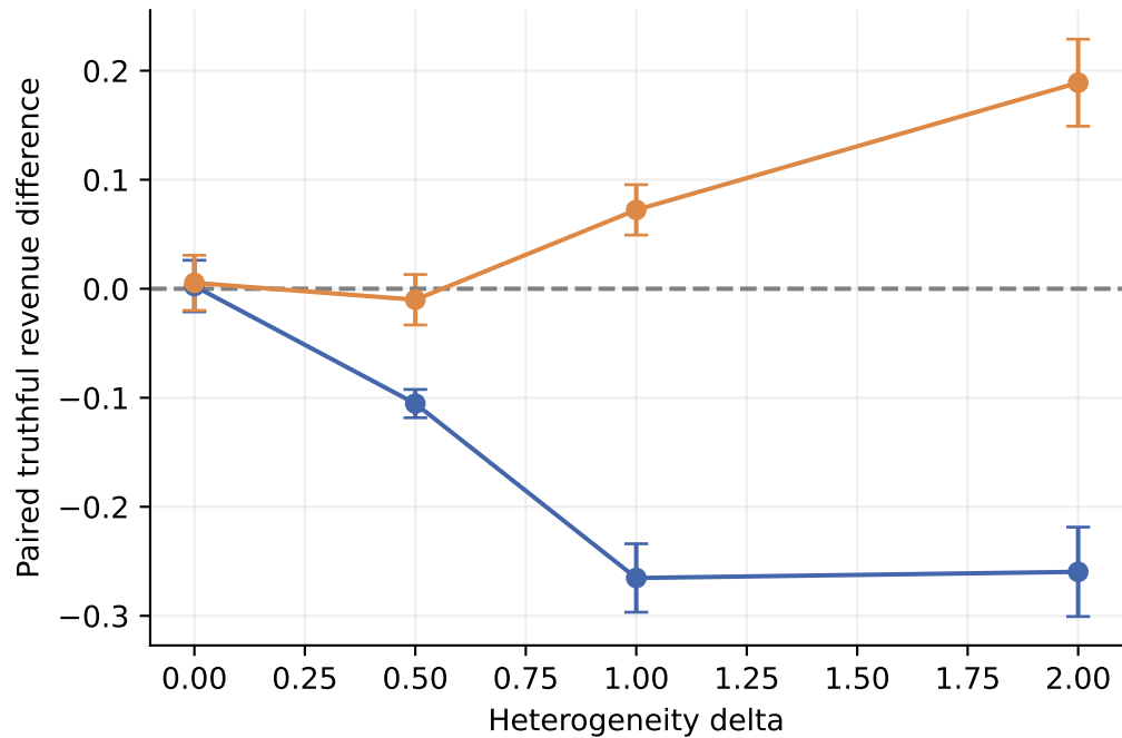
E4 paired differences — descriptive 95% t intervals, five seeds
