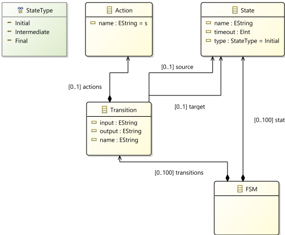
Figure 1. The ecore diagram of a FSM.
