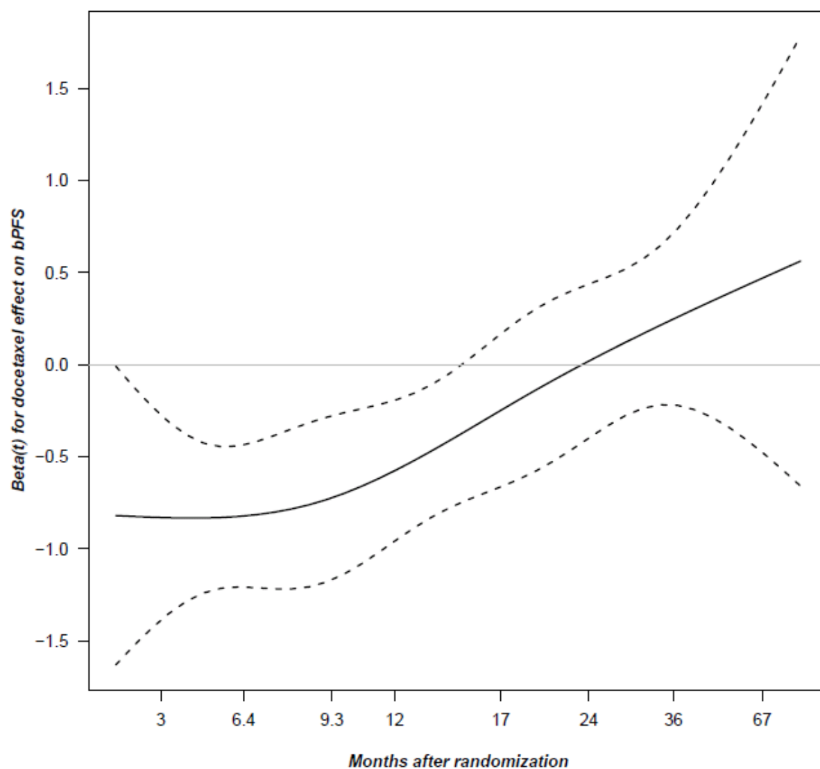
Supplementary figure 2: log (HR) of docetaxel effect on bPFS over time.
