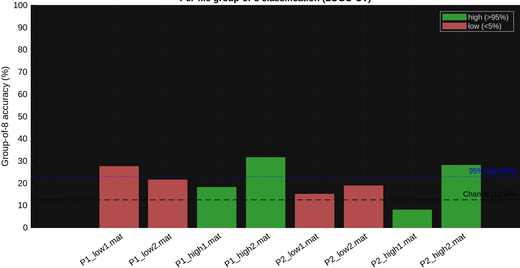
Per-file group-of-8 classification (LOGO-CV)
