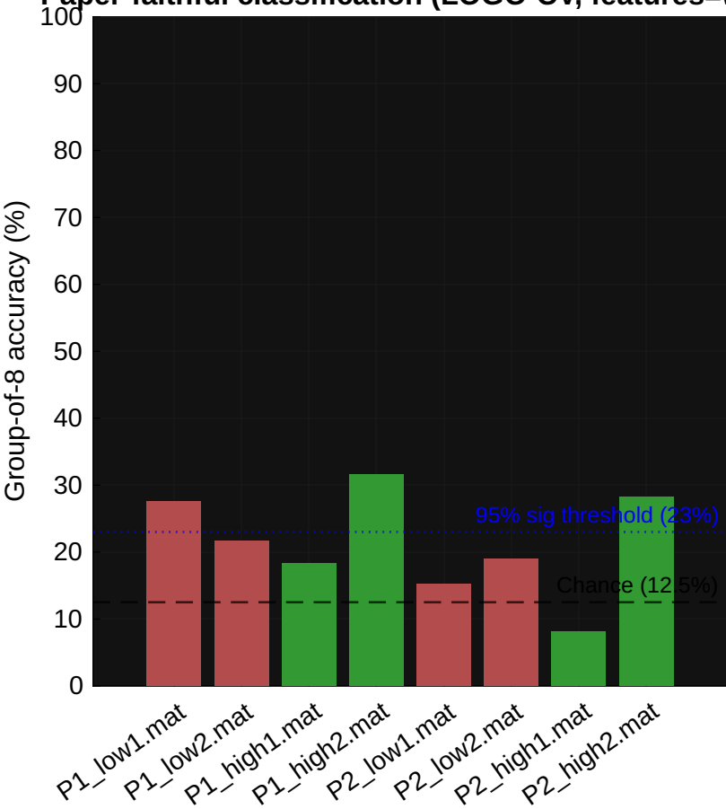
Paper-faithful classification (LOGO-CV, features=win)
