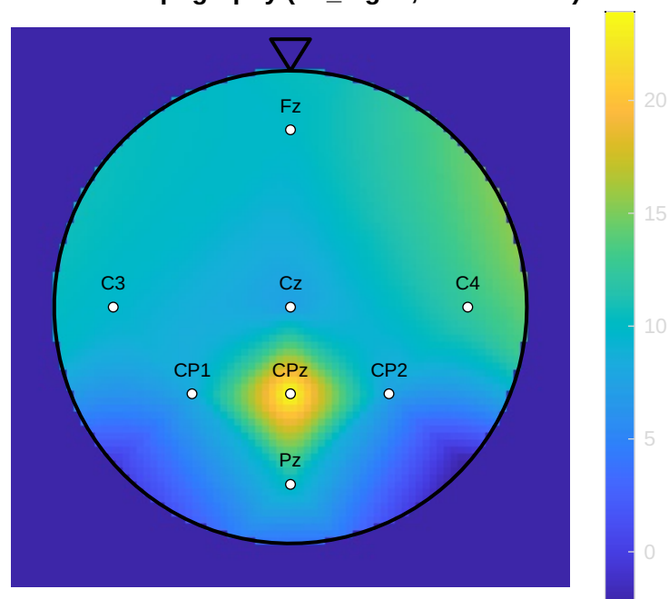
Activation topography (P2_high2, 200–500 ms)
