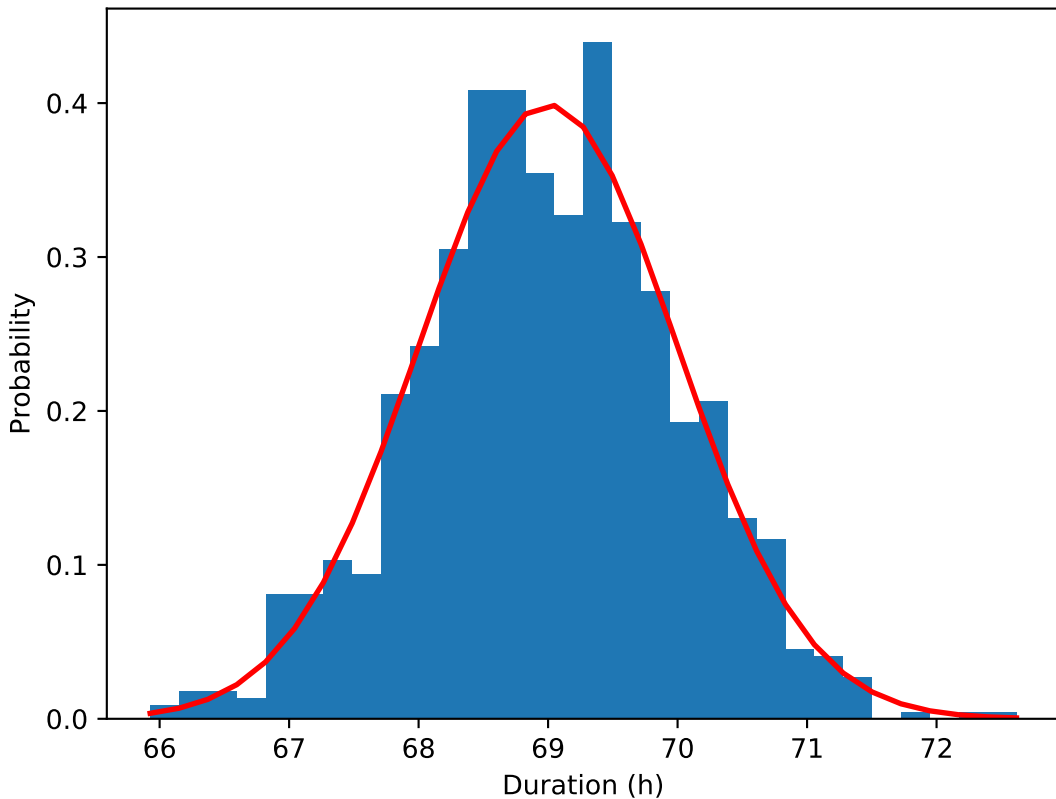
Durations under normal distribution ( \mu=69 , \sigma=1 )
