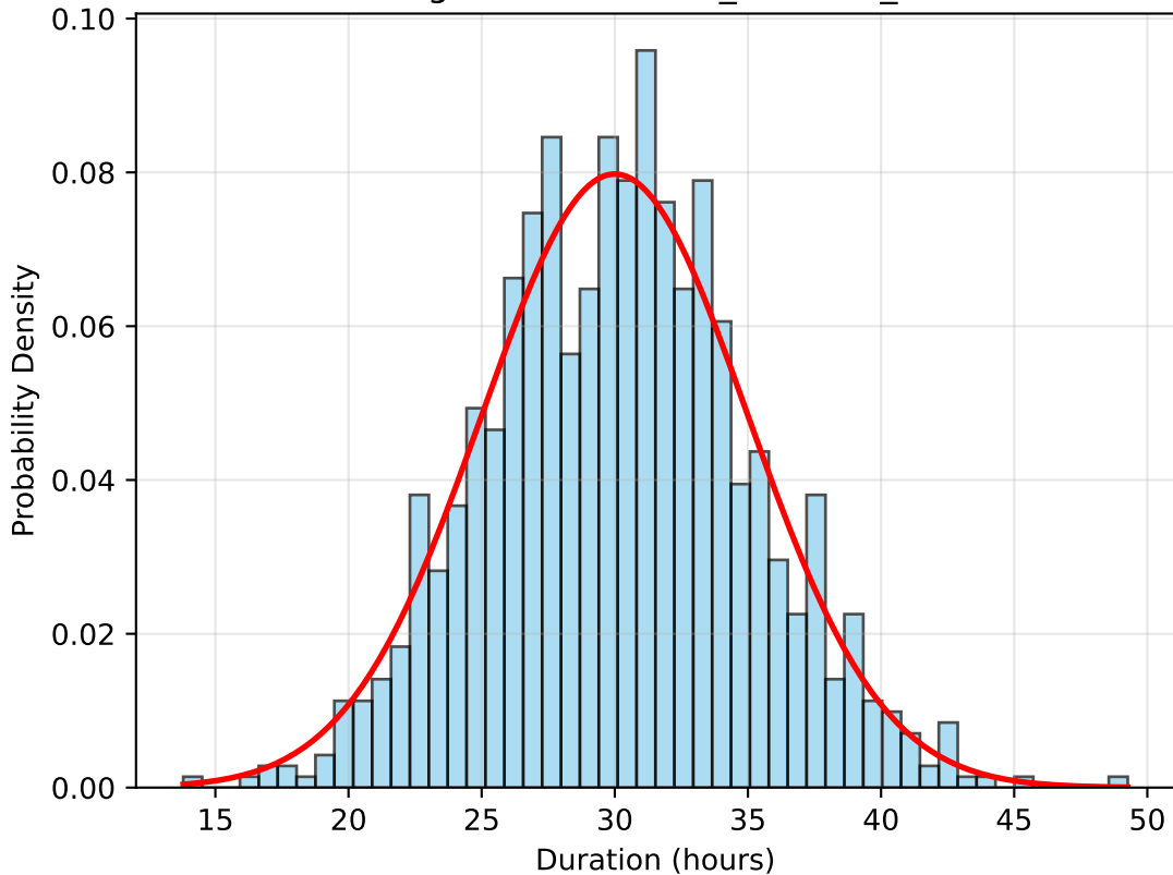
Normal Distribution ( \mu=30 , \sigma=5 ) Configuration: normal_mean30_std5
