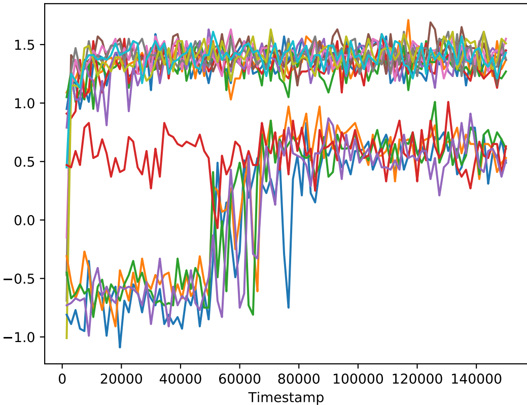
Average Reward
