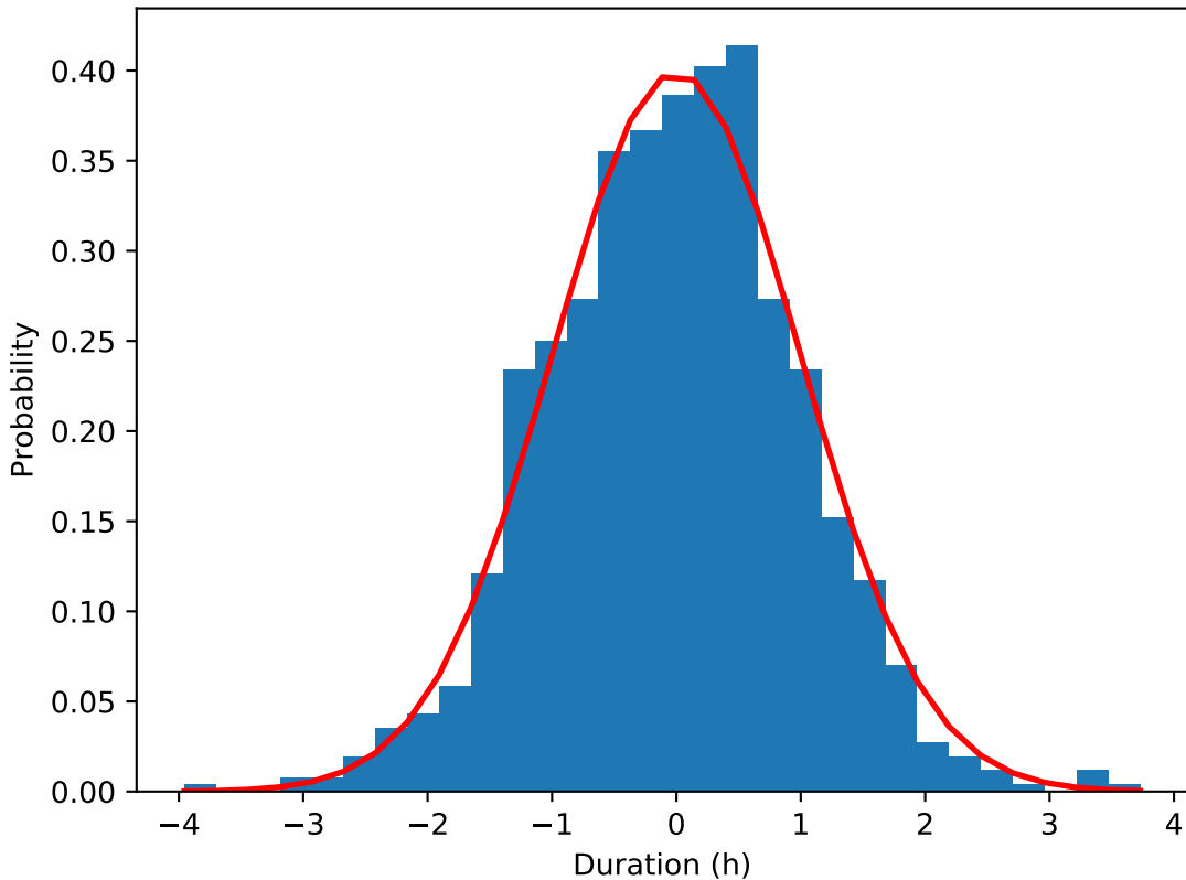
Durations under normal distribution ( \mu=0 , \sigma=1 )
