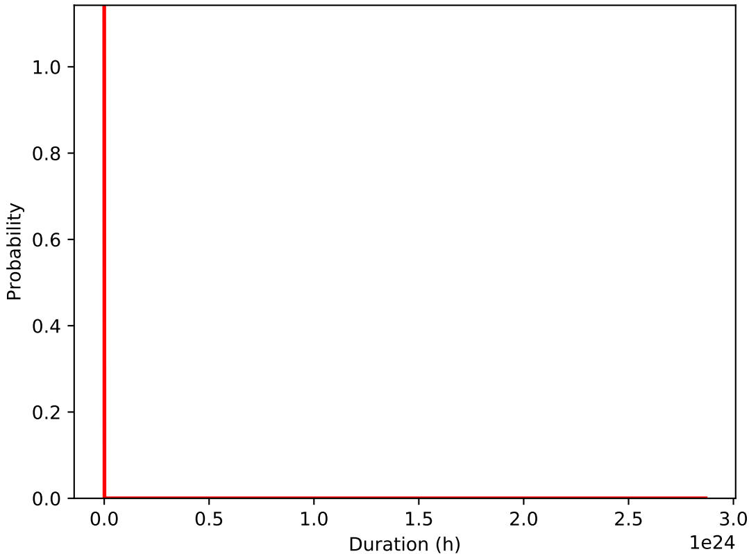
Durations under lognormal distribution ( \mu=40 , \sigma=5 )
