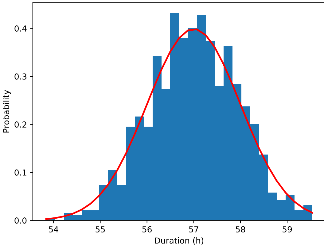
Durations under normal distribution ( \mu=57 , \sigma=1 )
