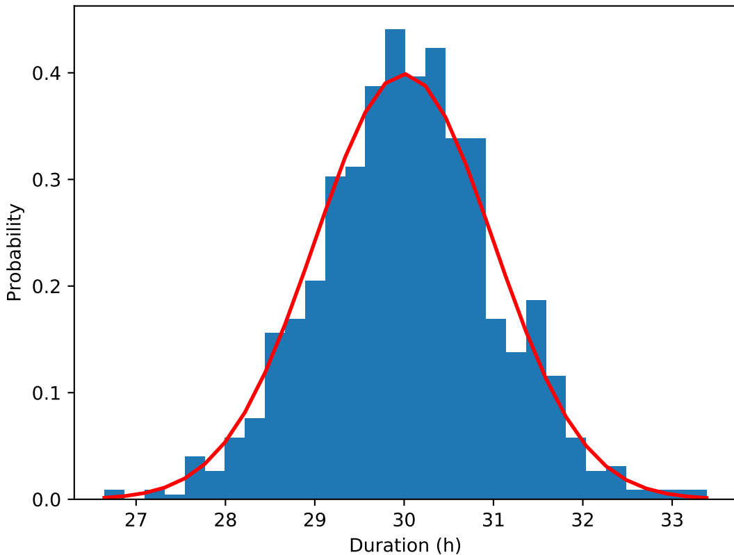
Durations under normal distribution ( \mu=30 , \sigma=1 )
