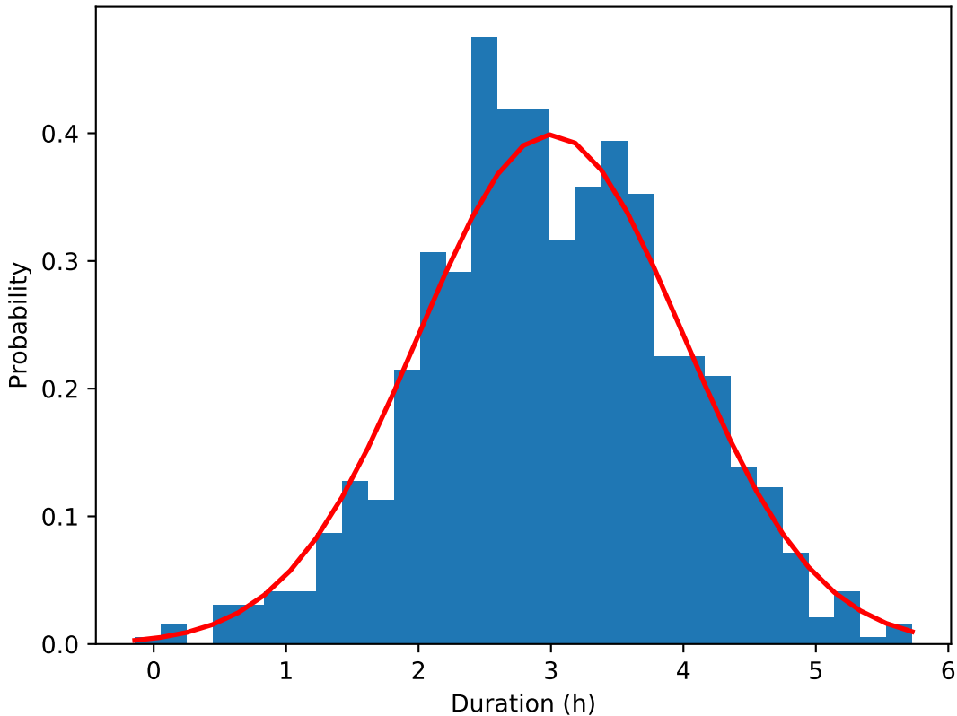
Durations under normal distribution ( \mu=3 , \sigma=1 )
