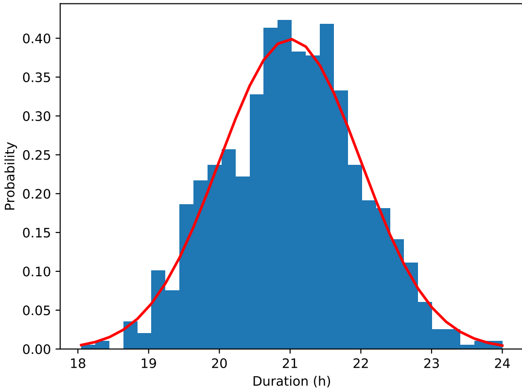
Durations under normal distribution ( \mu=21 , \sigma=1 )
