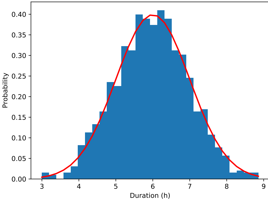
Durations under normal distribution ( \mu=6 , \sigma=1 )
