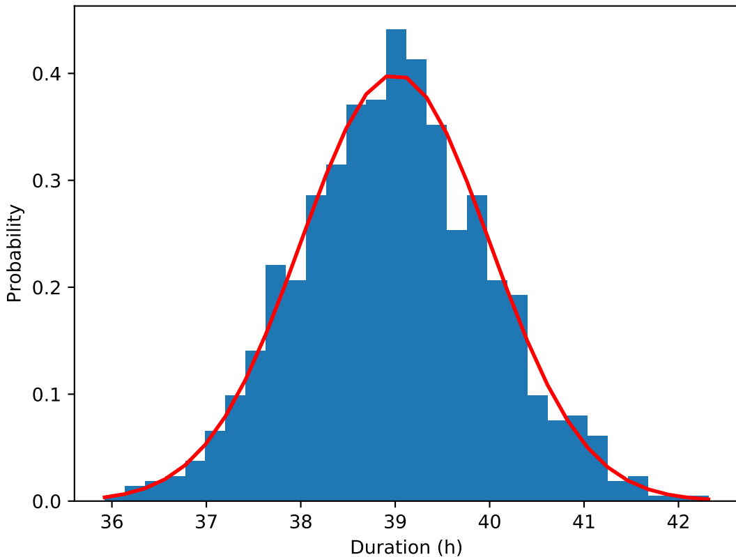
Durations under normal distribution ( \mu=39 , \sigma=1 )
