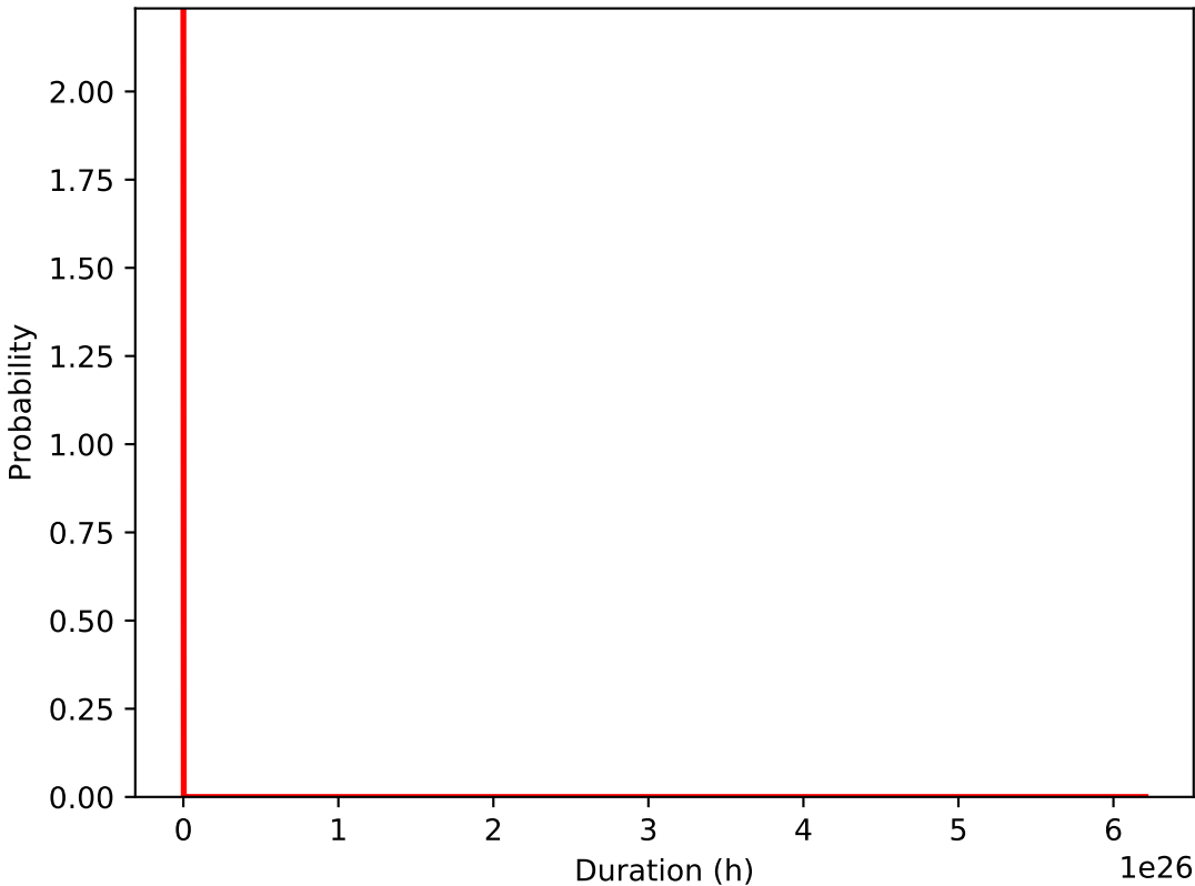
Durations under lognormal distribution ( \mu=40 , \sigma=5 )
