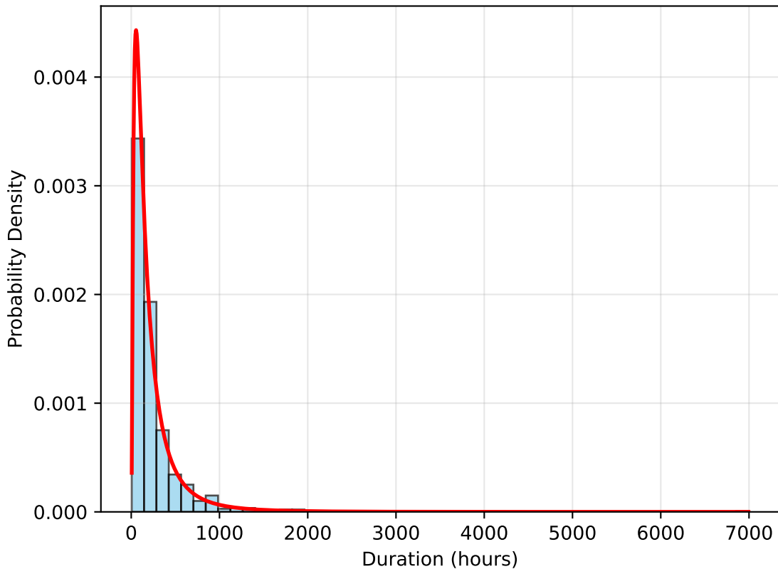
Lognormal Distribution ( \mu=5 , \sigma=1 ) Configuration: lognormal_mu5_sigma1
