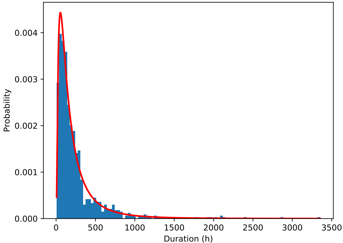
Durations under lognormal distribution ( \mu=5 , \sigma=1 )
