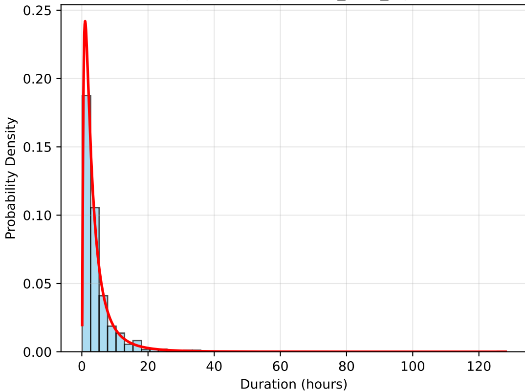
Lognormal Distribution ( \mu=1 , \sigma=1 ) Configuration: lognormal_mu1_sigma1
