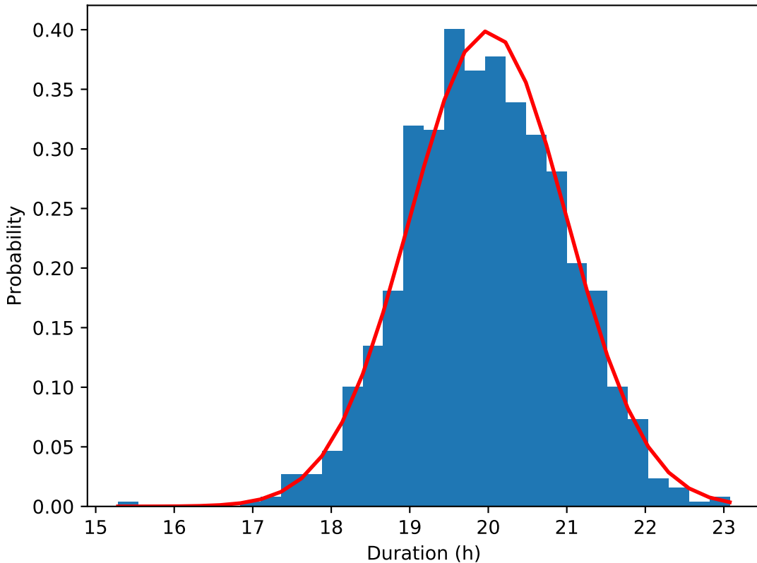
Durations under normal distribution ( \mu=20 , \sigma=1 )
