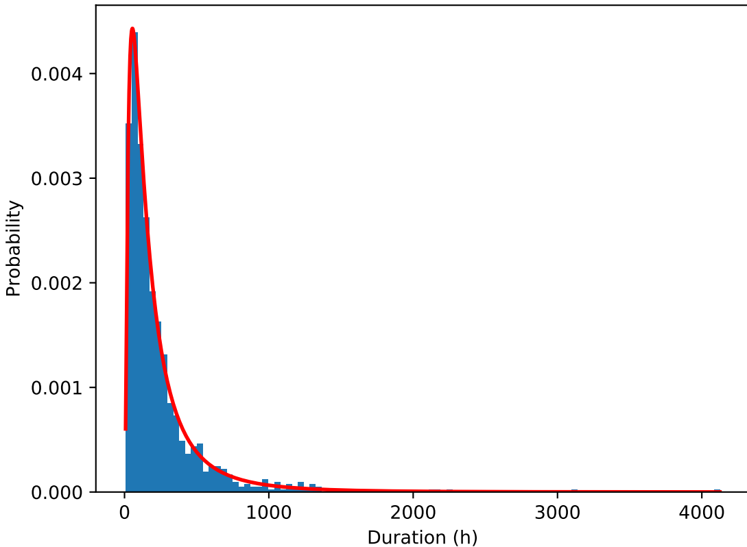
Durations under lognormal distribution ( \mu=5 , \sigma=1 )
