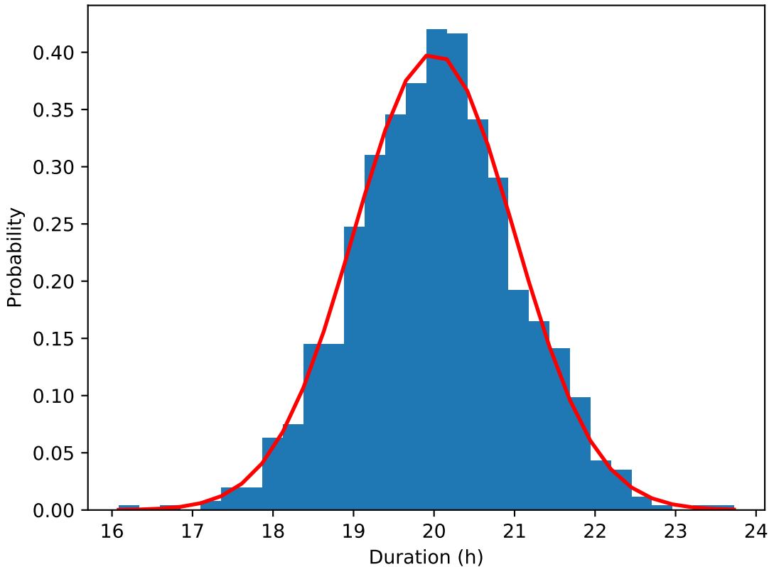
Durations under normal distribution ( \mu=20 , \sigma=1 )
