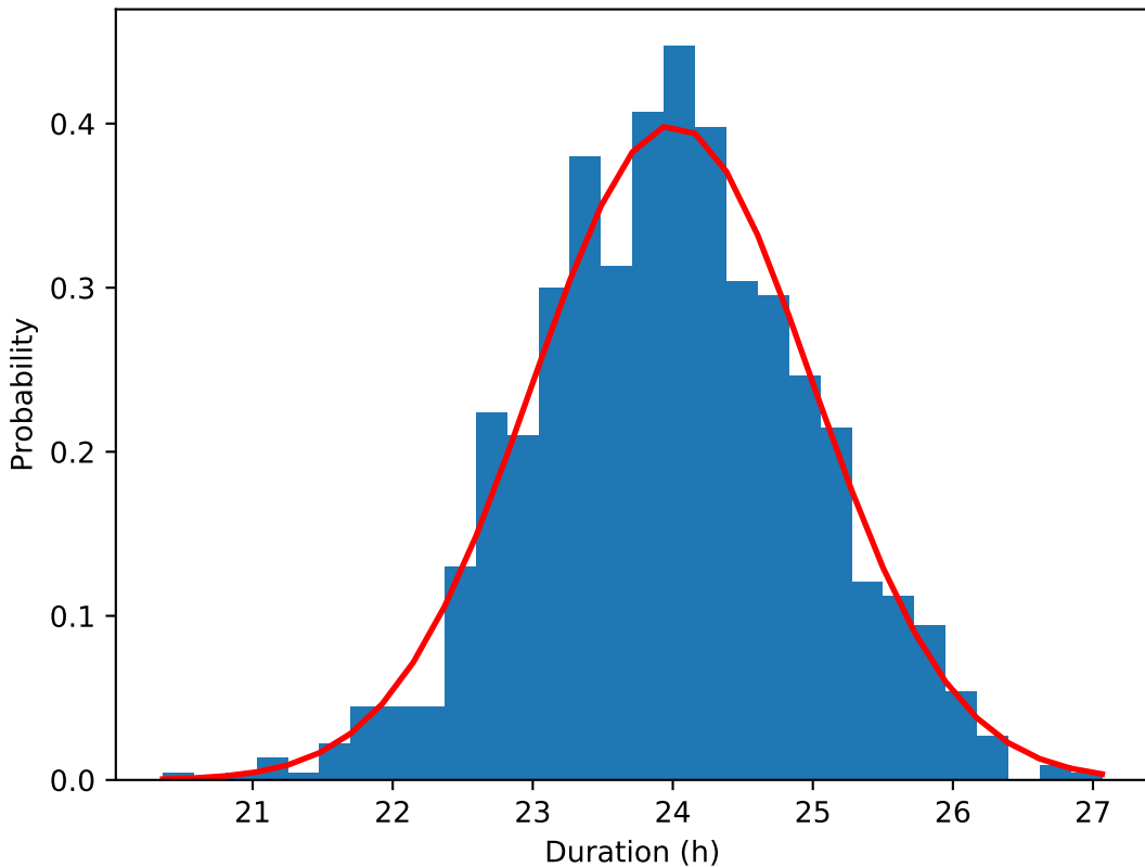
Durations under normal distribution ( \mu=24 , \sigma=1 )
