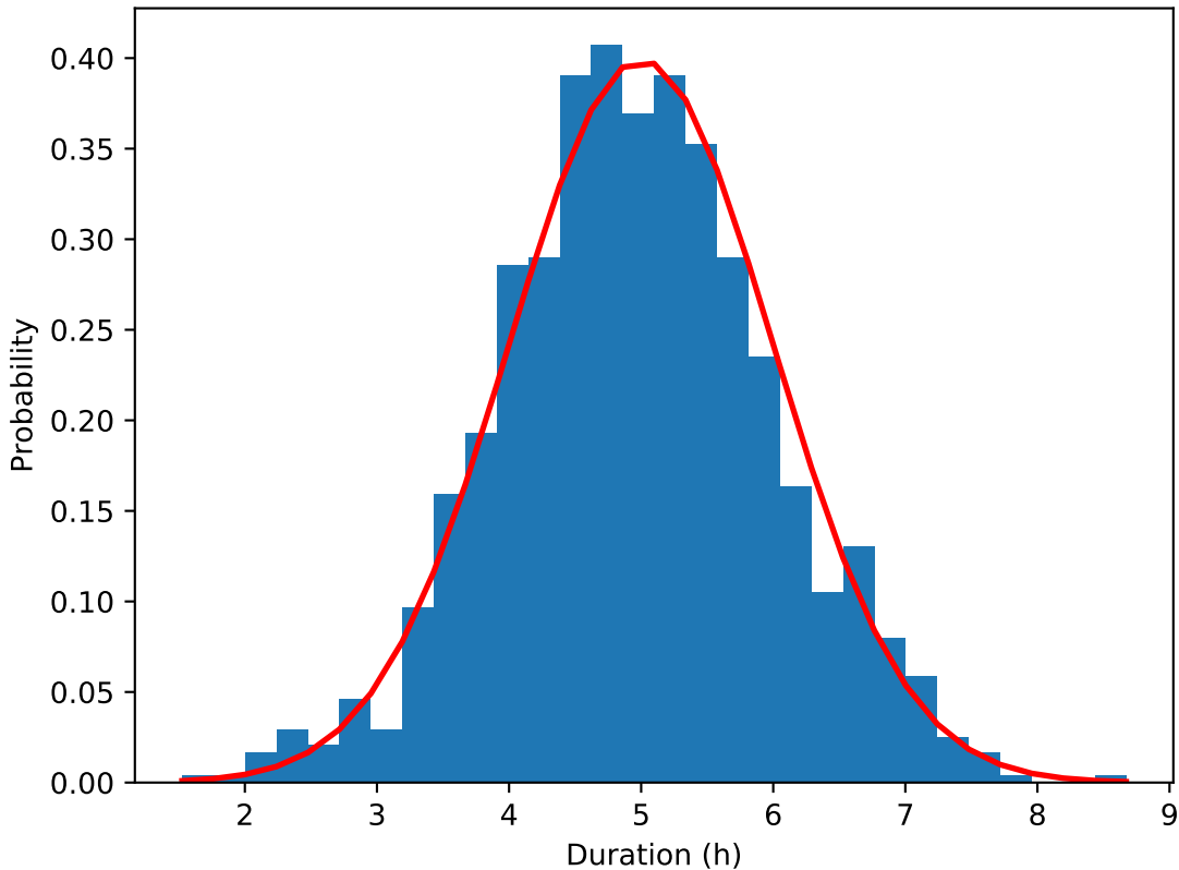
Durations under normal distribution ( \mu=5 , \sigma=1 )
