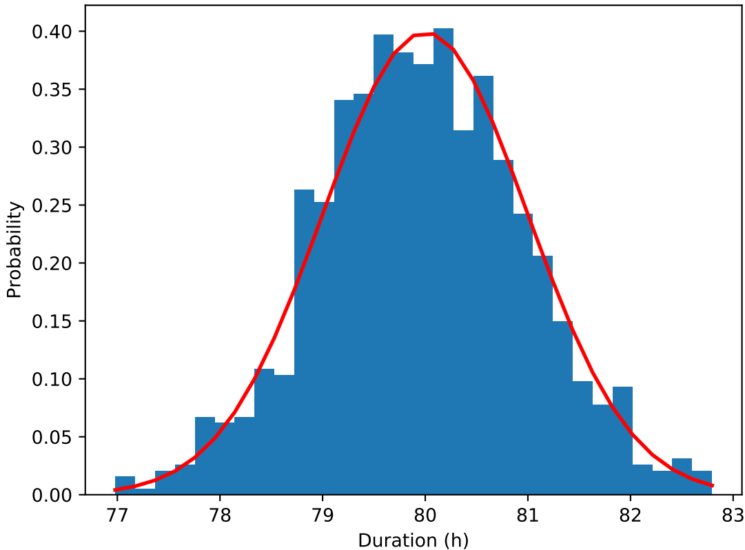
Durations under normal distribution ( \mu=80 , \sigma=1 )
