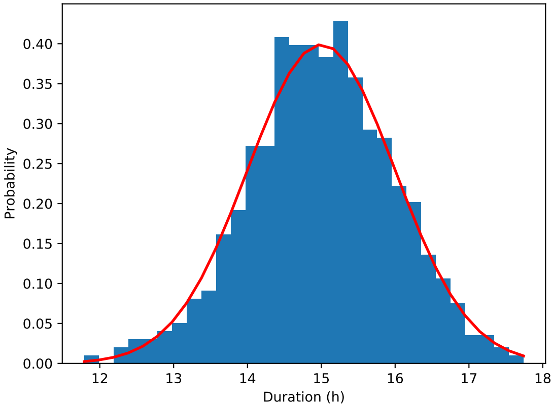
Durations under normal distribution ( \mu=15 , \sigma=1 )
