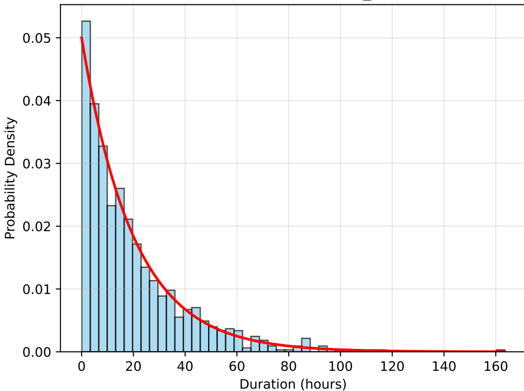
Exponential Distribution (scale=20) Configuration: exponential_scale20
