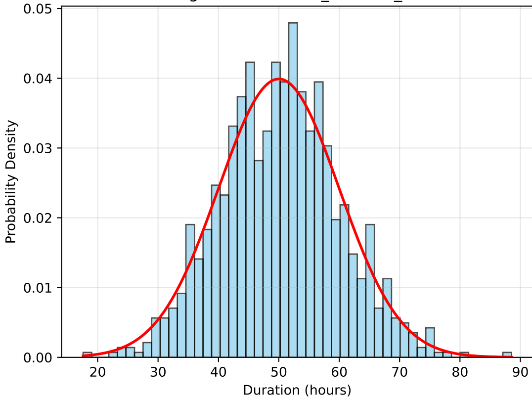
Normal Distribution ( \mu=50 , \sigma=10 ) Configuration: normal_mean50_std10
