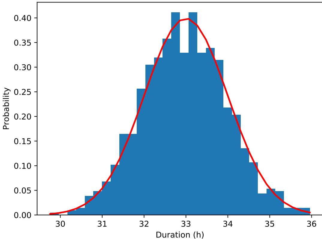
Durations under normal distribution ( \mu=33 , \sigma=1 )
