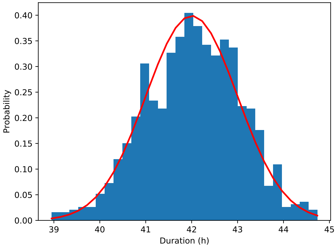
Durations under normal distribution ( \mu=42 , \sigma=1 )
