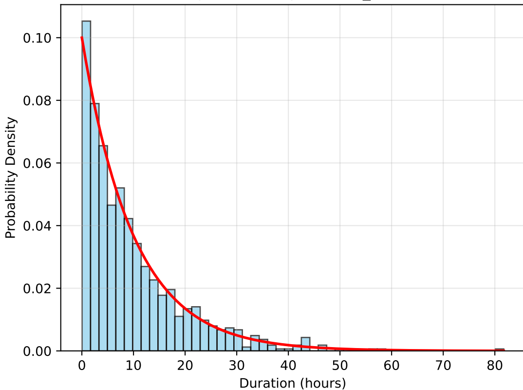
Exponential Distribution (scale=10) Configuration: exponential_scale10
