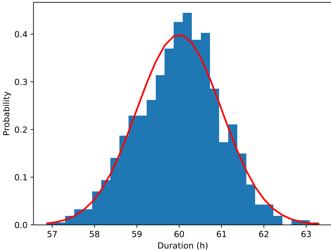
Durations under normal distribution ( \mu=60 , \sigma=1 )
