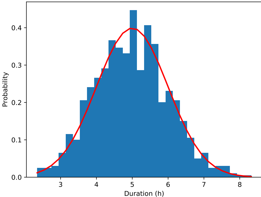
Durations under normal distribution ( \mu=5 , \sigma=1 )
