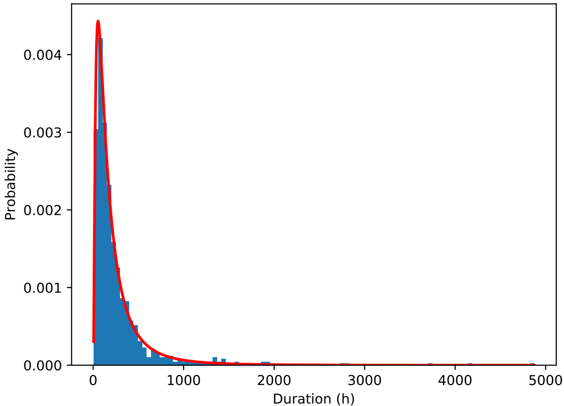
Durations under lognormal distribution ( \mu=5 , \sigma=1 )
