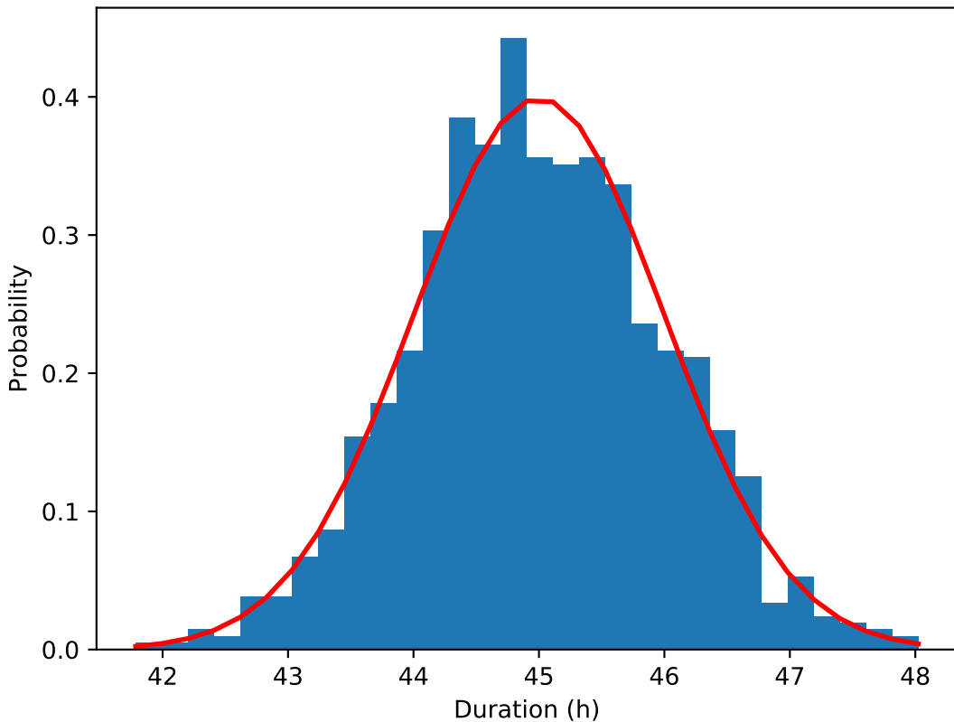
Durations under normal distribution ( \mu=45 , \sigma=1 )
