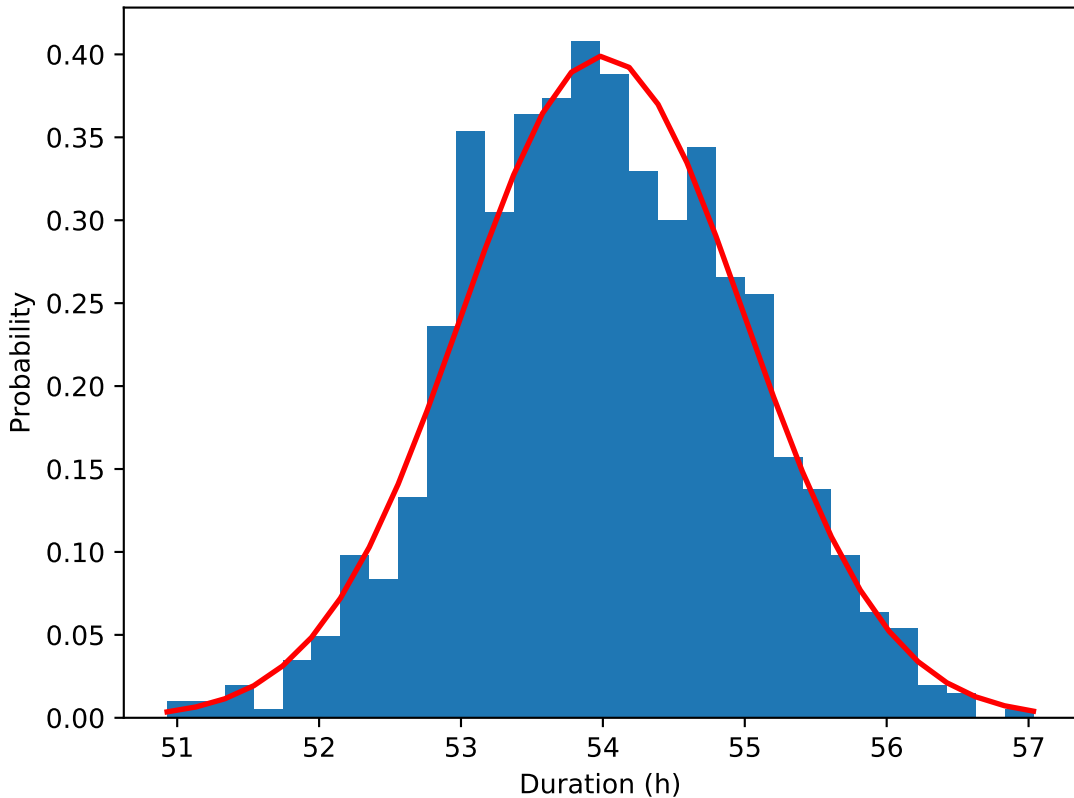
Durations under normal distribution ( \mu=54 , \sigma=1 )
