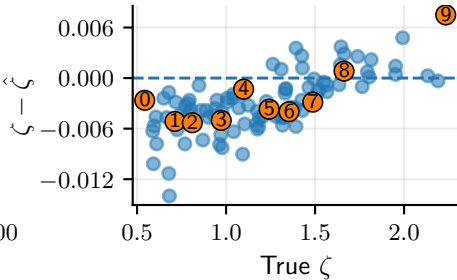
(c) FNO Residuals \hat{\mathcal{G}}_{\text{LS}}
