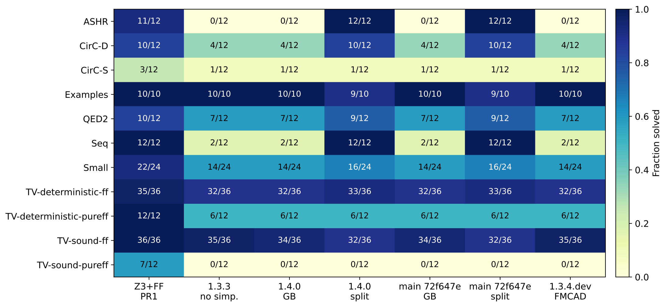
Coverage by family · the same 190 inputs in every column
