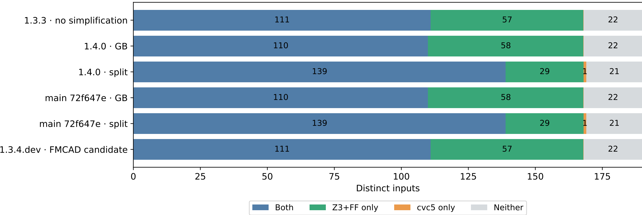
Which inputs does Z3+FF solve compared with each cvc5 configuration?
