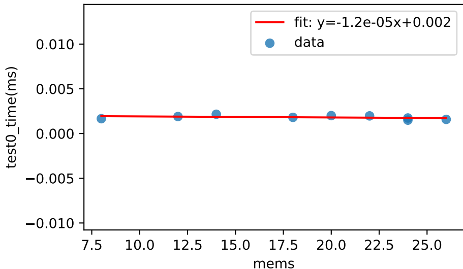
binsearch: mems vs. test0_time(ms) Pearson r=-0.335 , R^2=0.112
