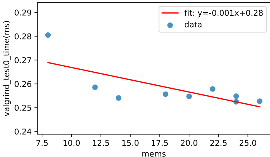
binsearch: mems vs. valgrind_test0_time(ms) Pearson r=-0.730 , R^2=0.534
