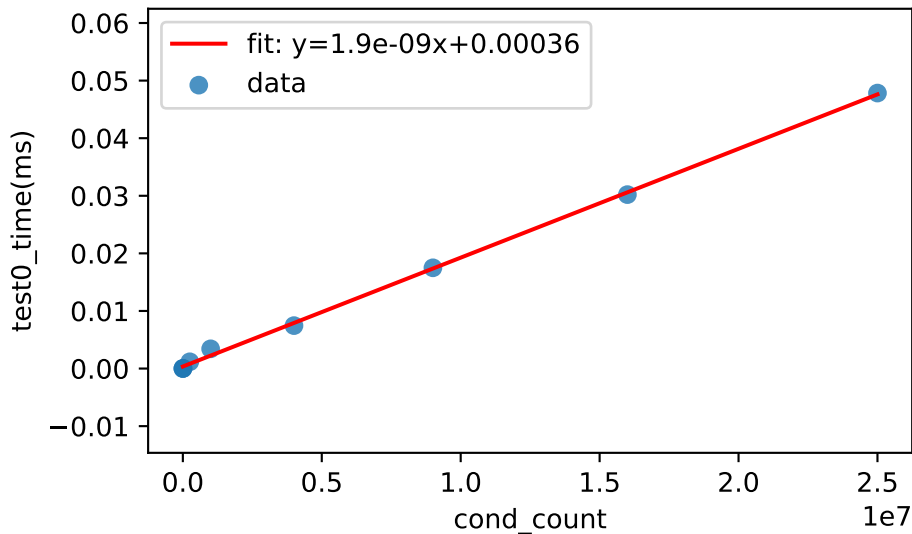
bubble: cond_count vs. test0_time(ms) Pearson r=0.999 , R^2=0.999
