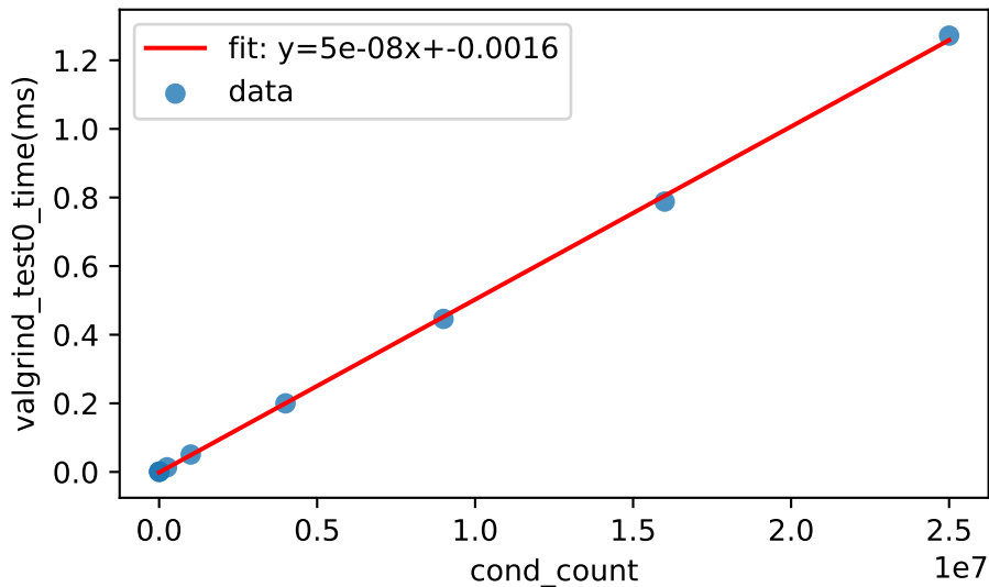
bubble: cond_count vs. valgrind_test0_time(ms) Pearson r=1.000 , R^2=1.000
