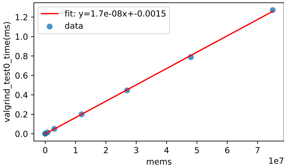
bubble: mems vs. valgrind_test0_time(ms) Pearson r=1.000 , R^2=1.000
