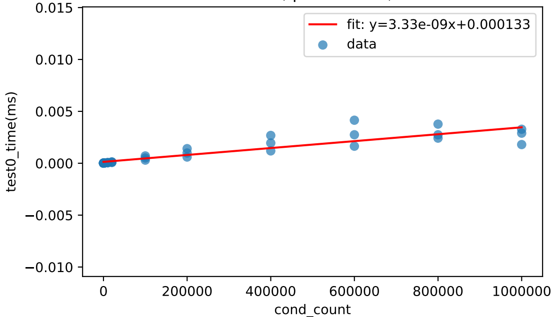
cond_count vs. test0_time(ms) Pearson r=0.899 , p=7.88e-15 , R^2=0.808
