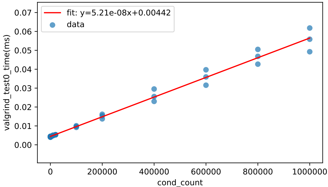
cond_count vs. valgrind_test0_time(ms) Pearson r=0.993 , p=1.23e-35 , R^2=0.986
