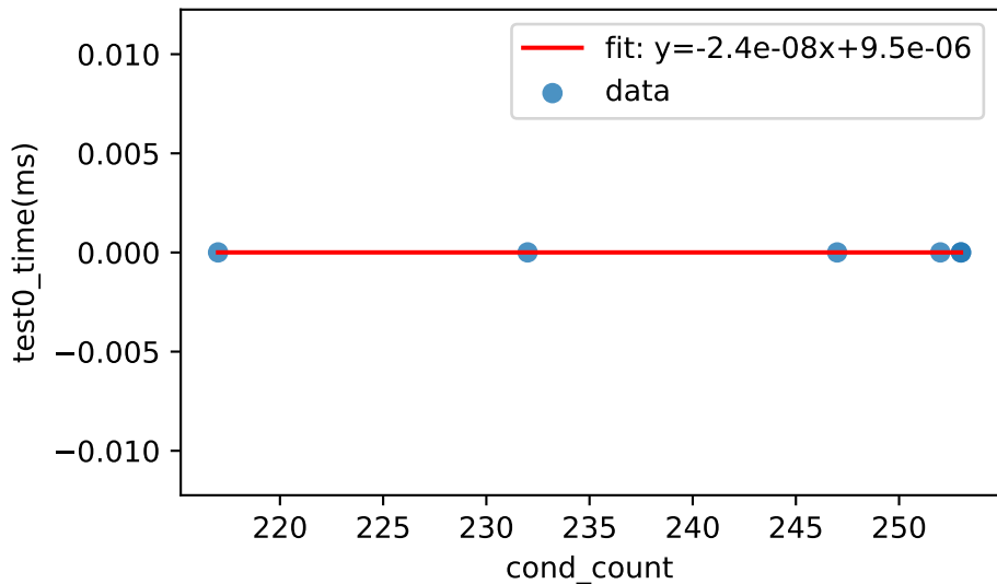
dijkstra: cond_count vs. test0_time(ms) Pearson r=-0.462 , R^2=0.213
