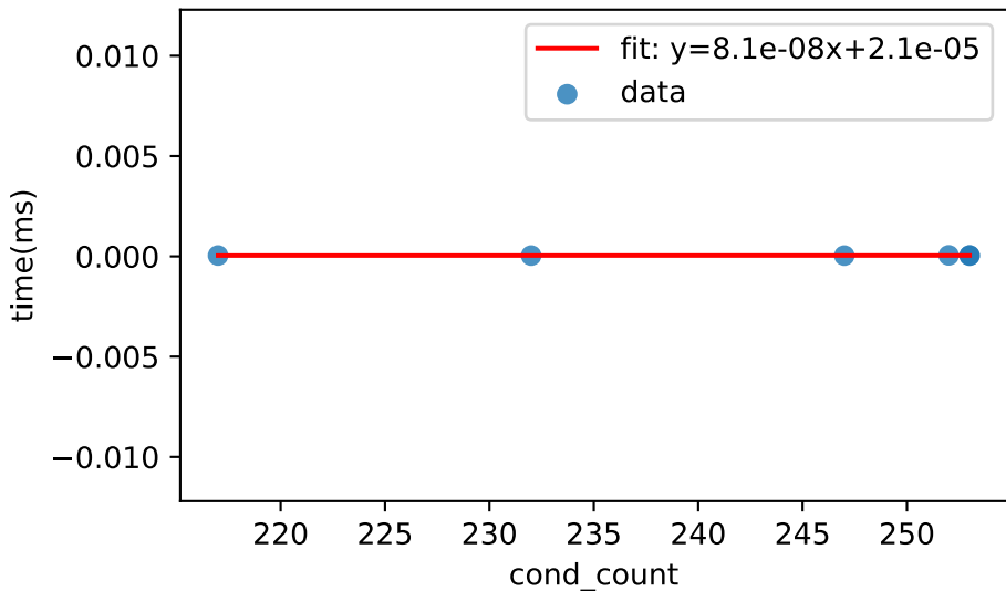
dijkstra: cond_count vs. time(ms) Pearson r=0.255 , R^2=0.065
