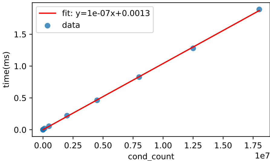
insertsort: cond_count vs. time(ms) Pearson r=1.000 , R^2=1.000
