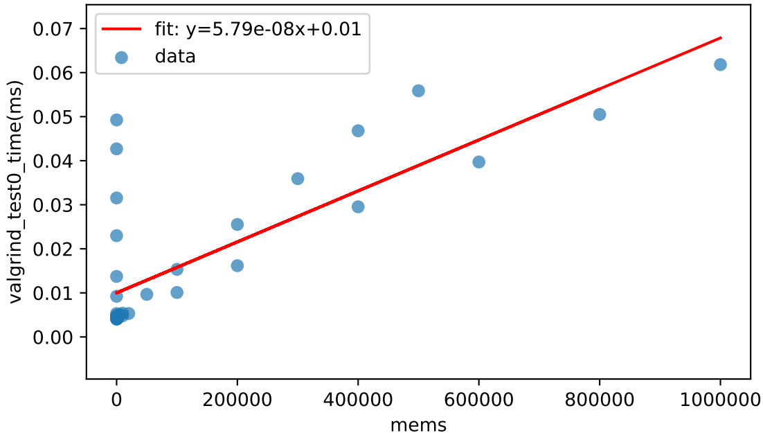
mems vs. valgrind_test0_time(ms) Pearson r=0.783 , p=3.98e-09 , R^2=0.612
