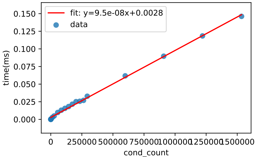
sieve: cond_count vs. time(ms) Pearson r=0.999 , R^2=0.997
