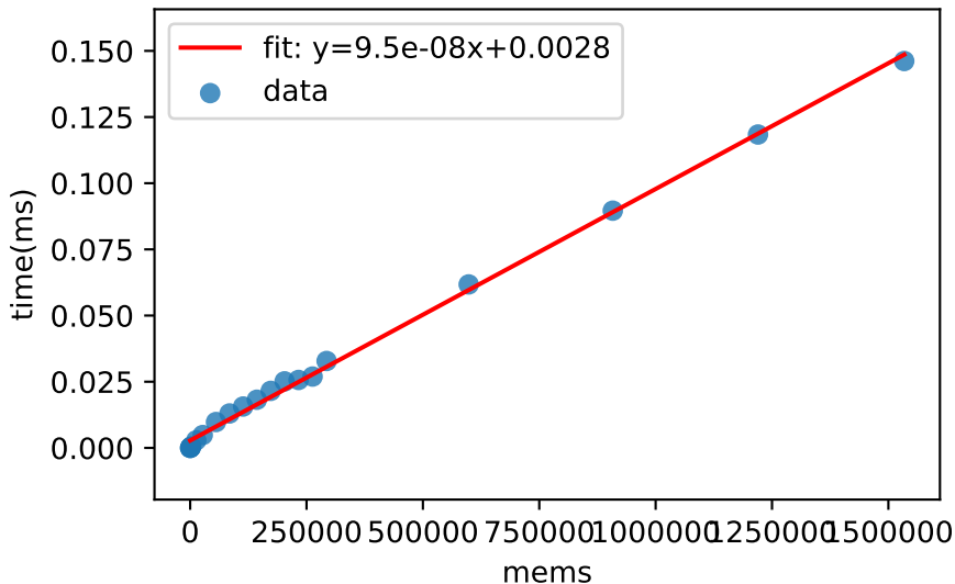
sieve: mems vs. time(ms) Pearson r=0.999 , R^2=0.997
