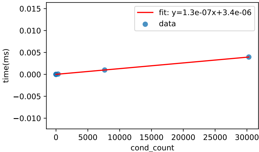
topo: cond_count vs. time(ms) Pearson r=1.000 , R^2=1.000
