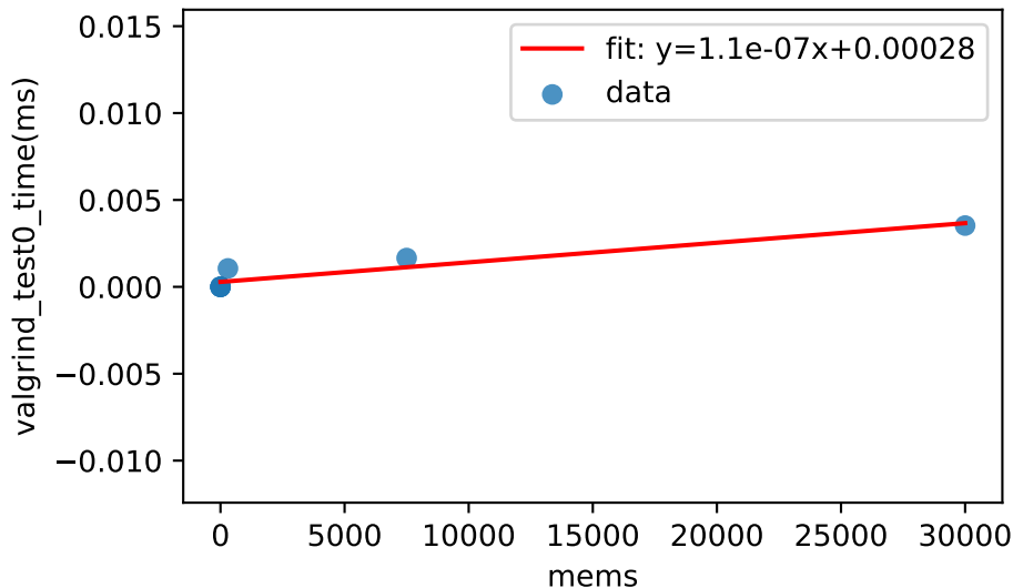
topo: mems vs. valgrind_test0_time(ms) Pearson r=0.944 , R^2=0.891
