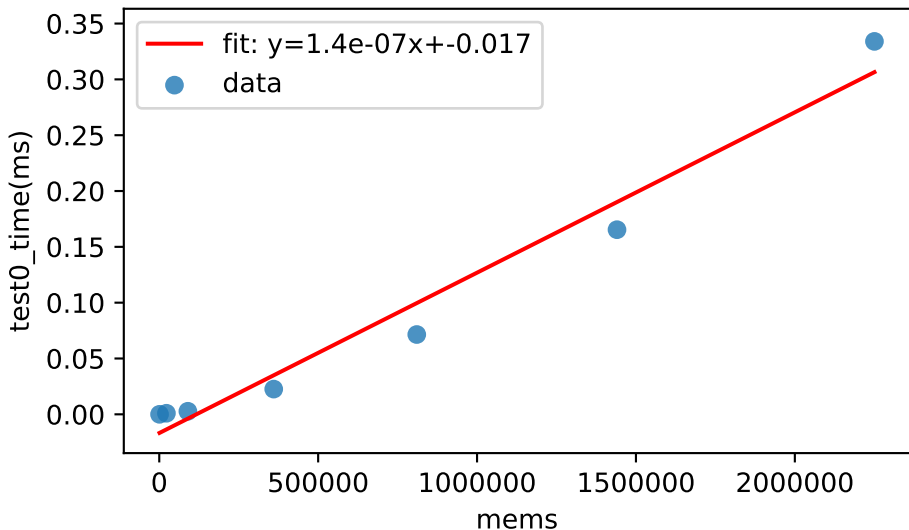
warshall: mems vs. test0_time(ms) Pearson r=0.985 , R^2=0.970
