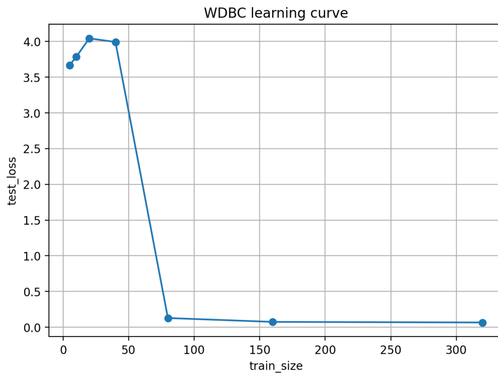
Figure 2: Learning Curve for WDBC
