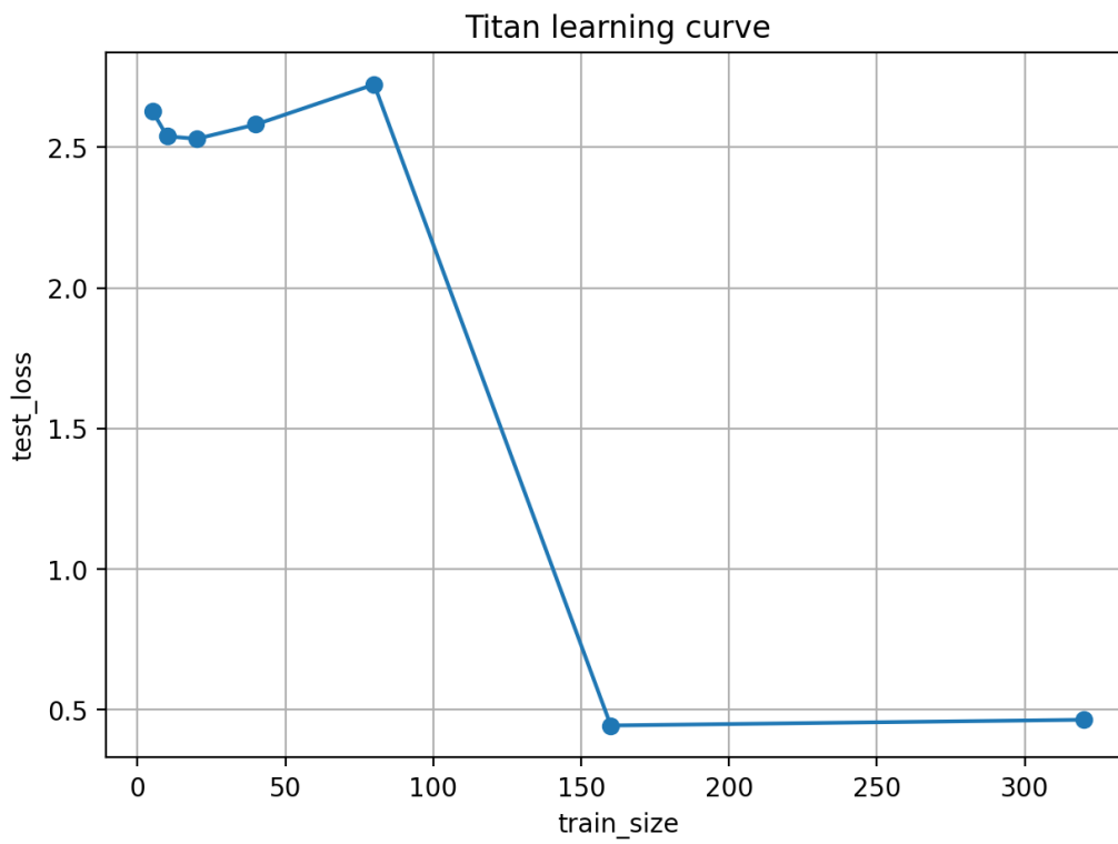
Figure 5: Learning Curve for Titanic
