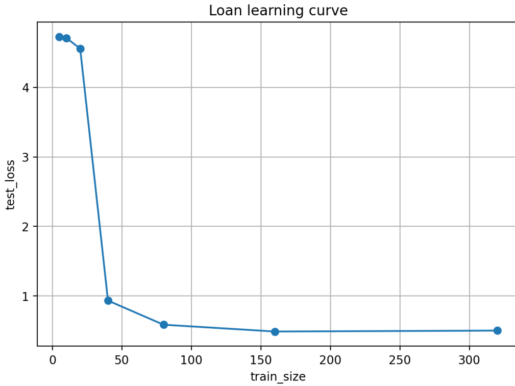
Figure 3: Learning Curve for Loan
