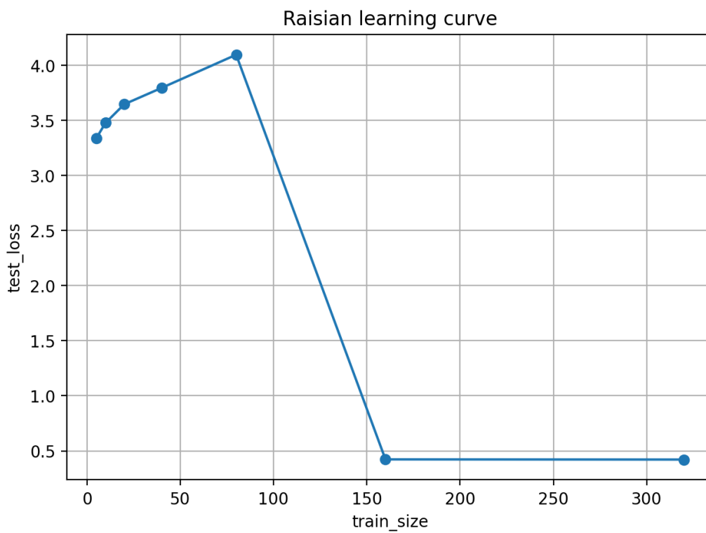
Figure 4: Learning Curve for Raisins
