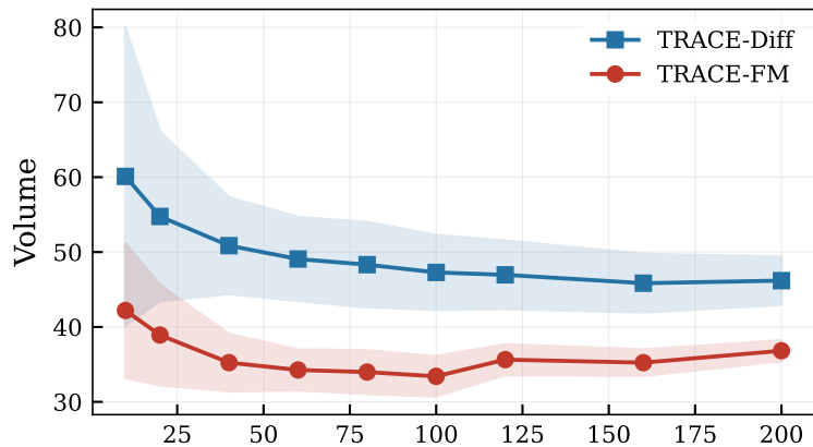
Pinwheel
