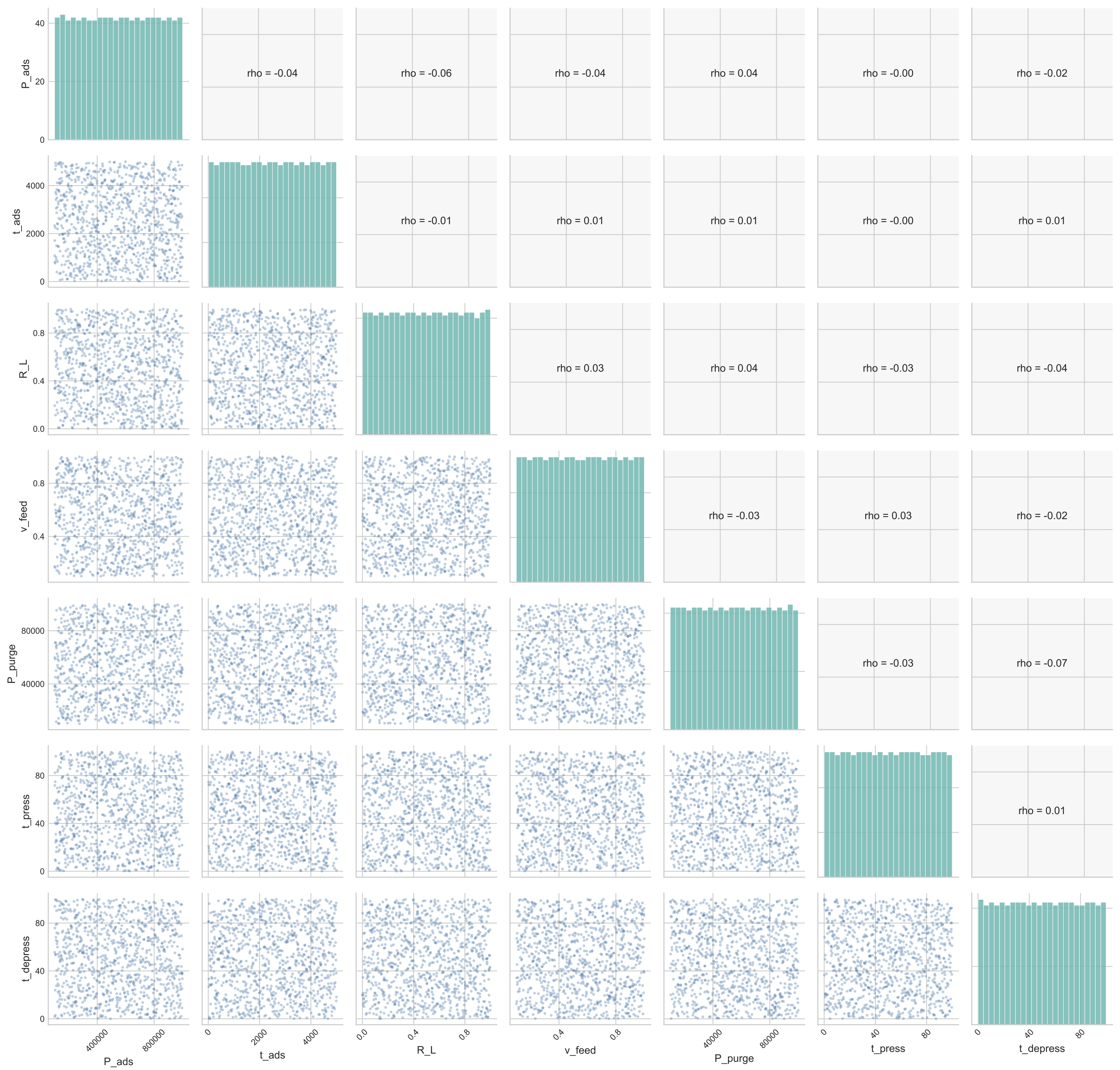
Pairwise Coverage of LHS Design Variables
