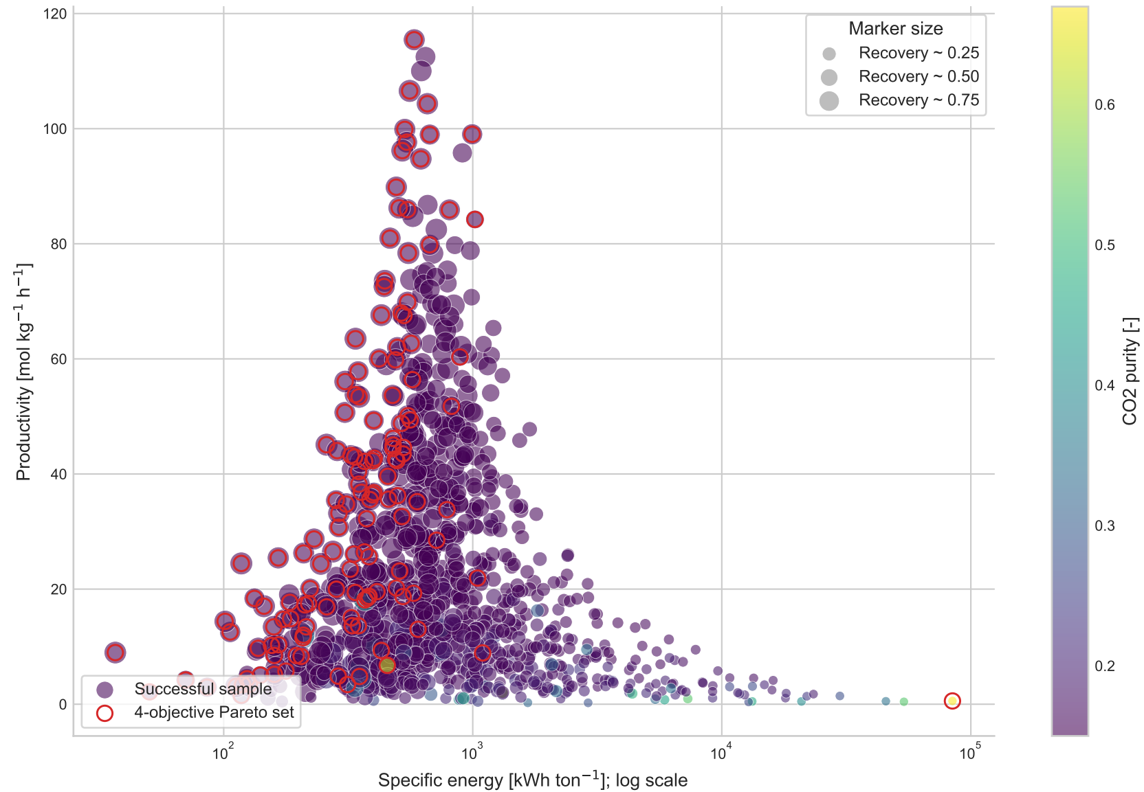
Four-Objective Pareto Set Projected onto Productivity-Energy Plane
