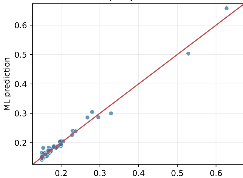
Productivity (R2=0.994)
