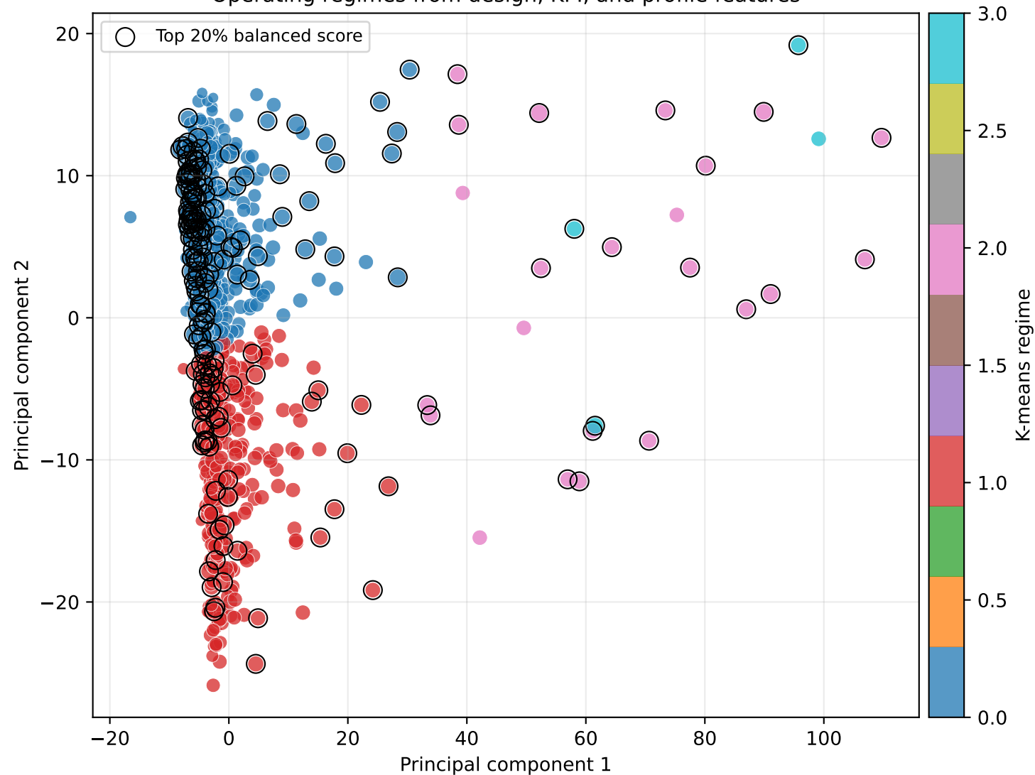
Operating regimes from design, KPI, and profile features
