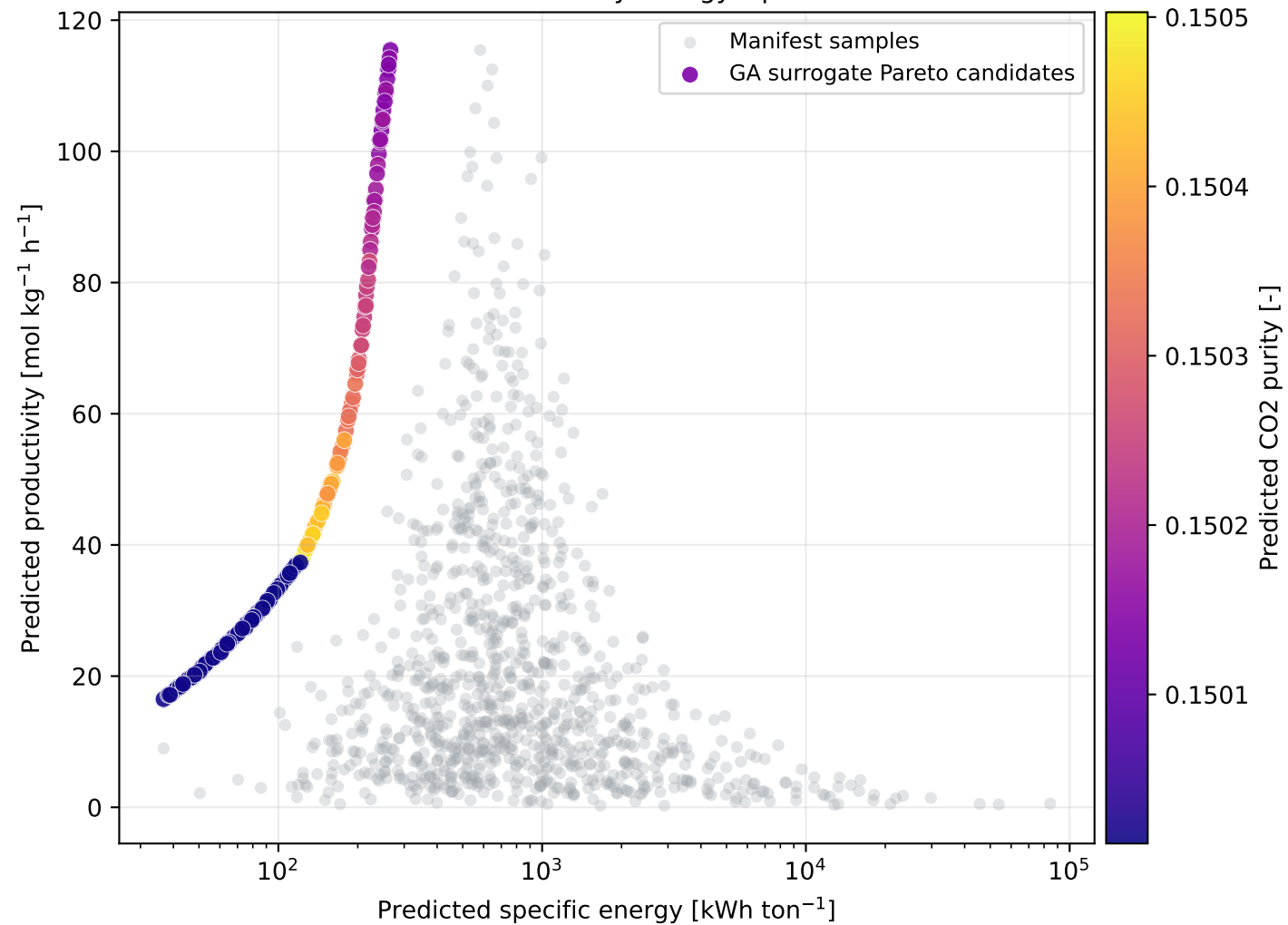
GA Front for Productivity-Energy Optimization
