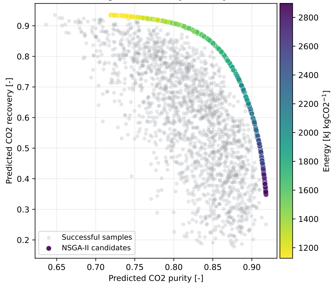
Surrogate Front: Purity-Recovery
