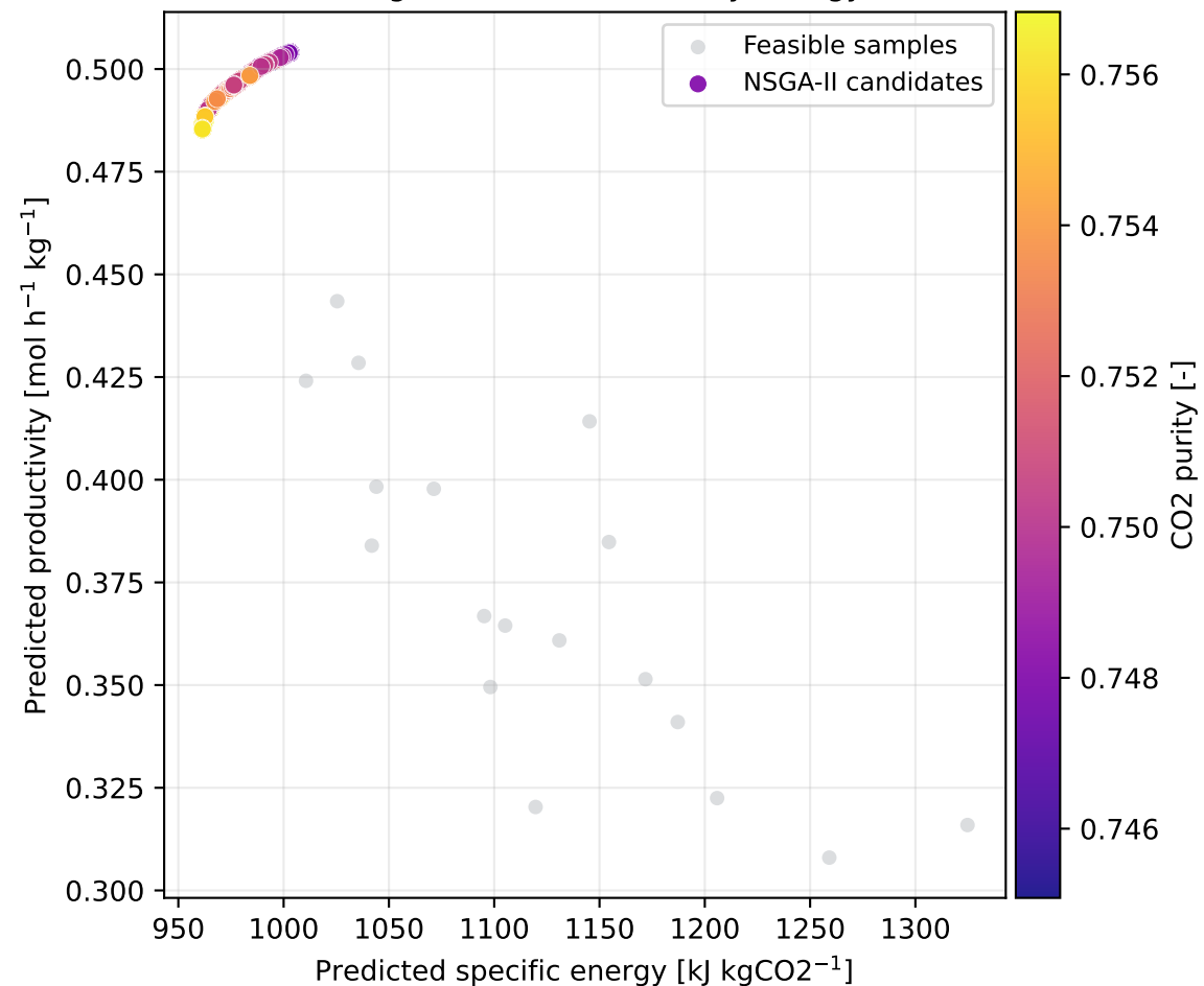
Surrogate Front: Productivity-Energy
