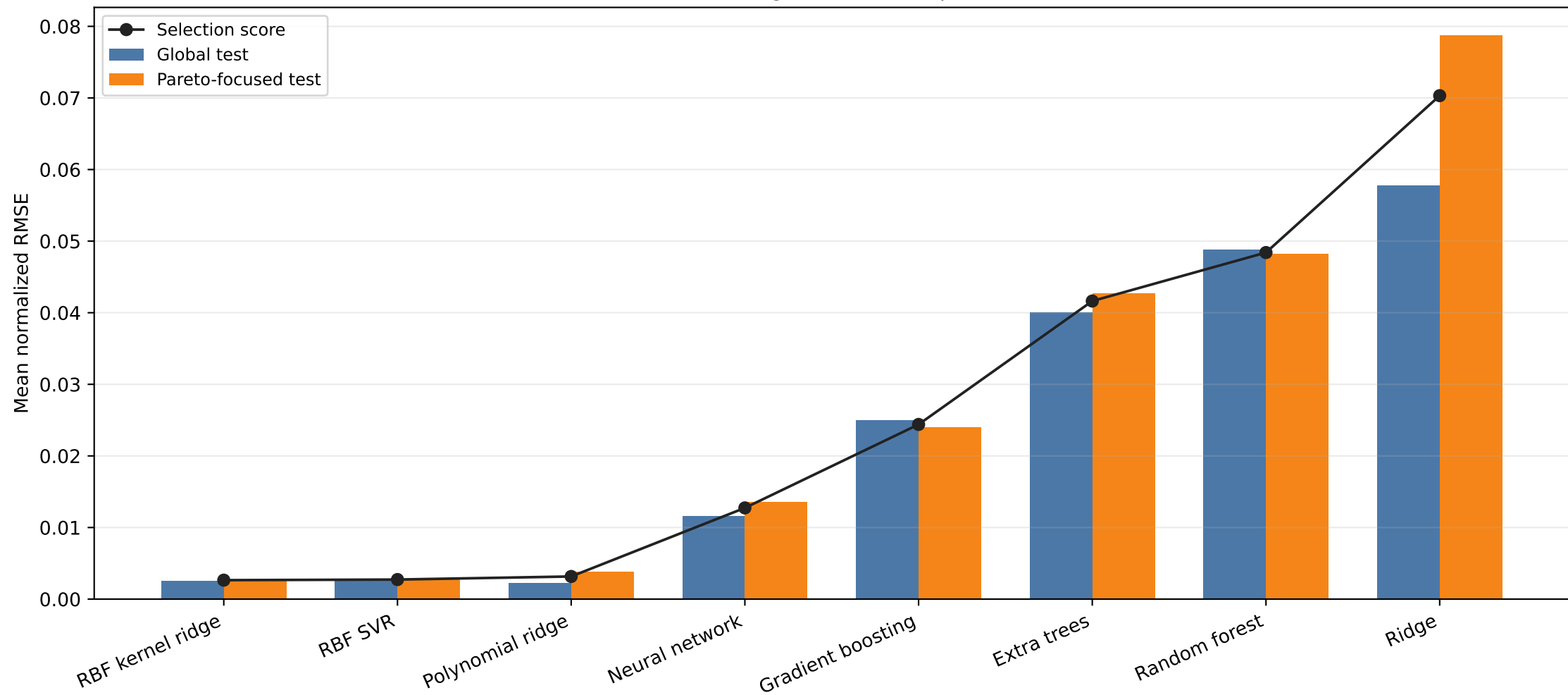
Tuned Surrogate Model Comparison
