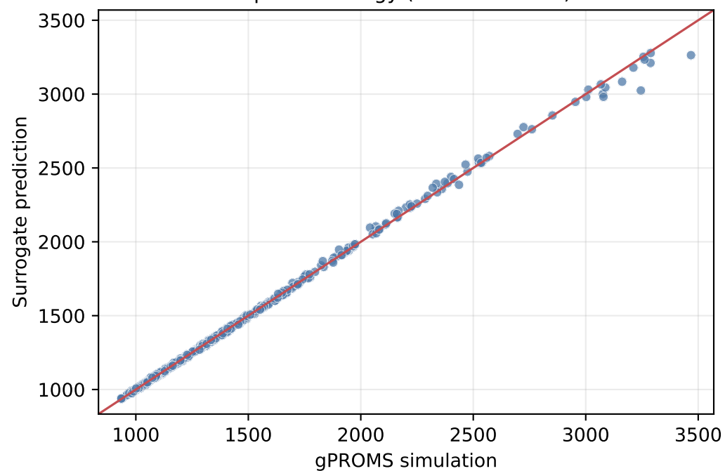
Specific energy (test R2=0.998)
