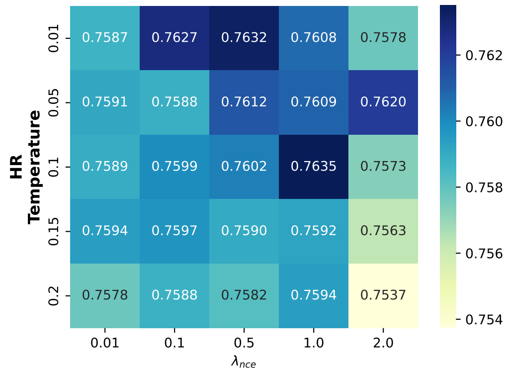
Dataset: AWM
