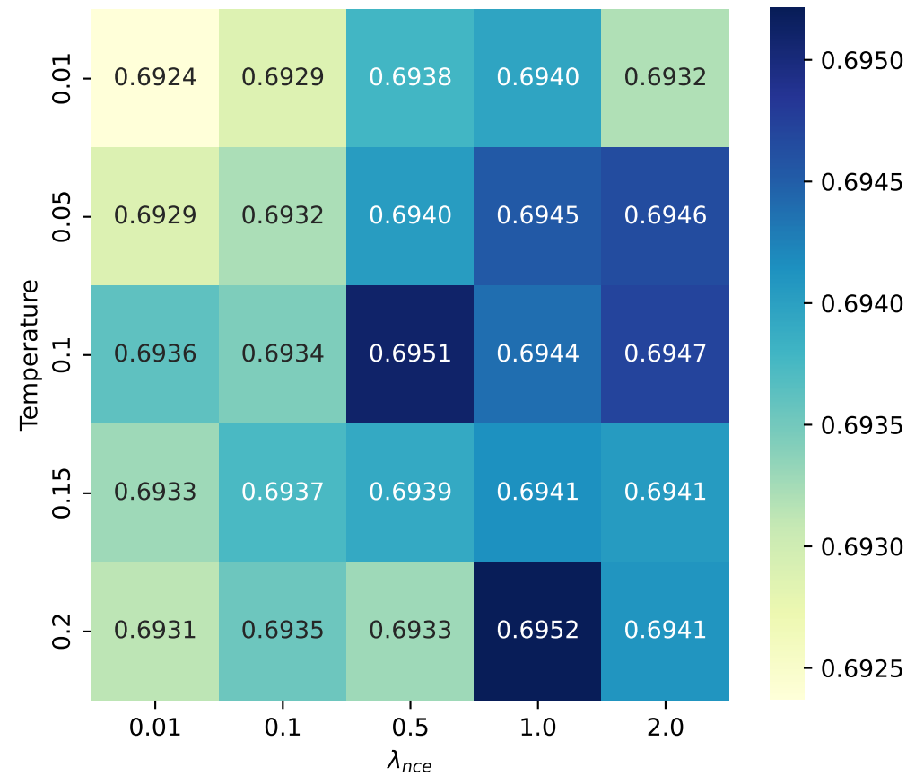
Dataset: HIP
