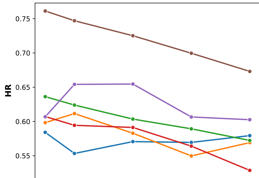
Dataset: AWM
