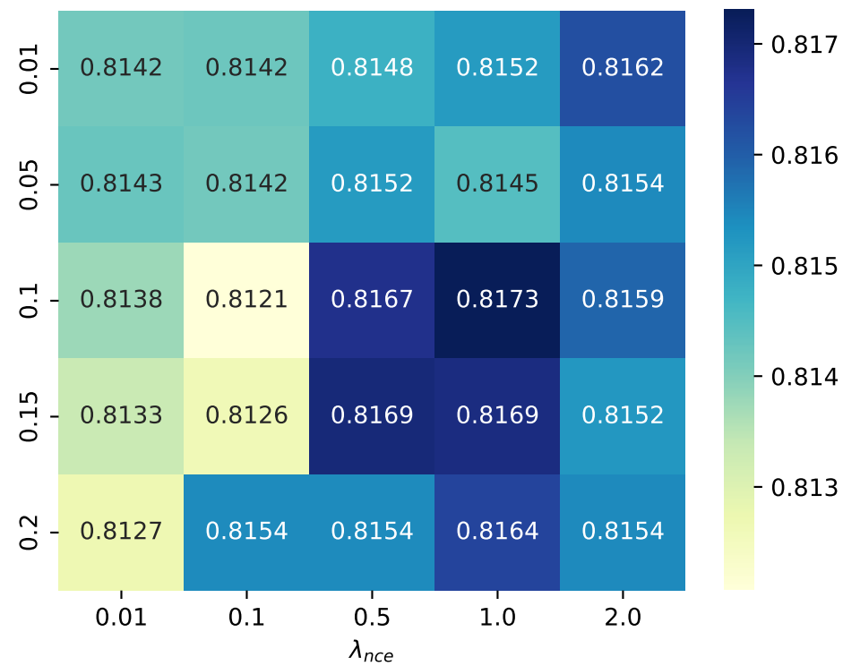
Dataset: HIP
