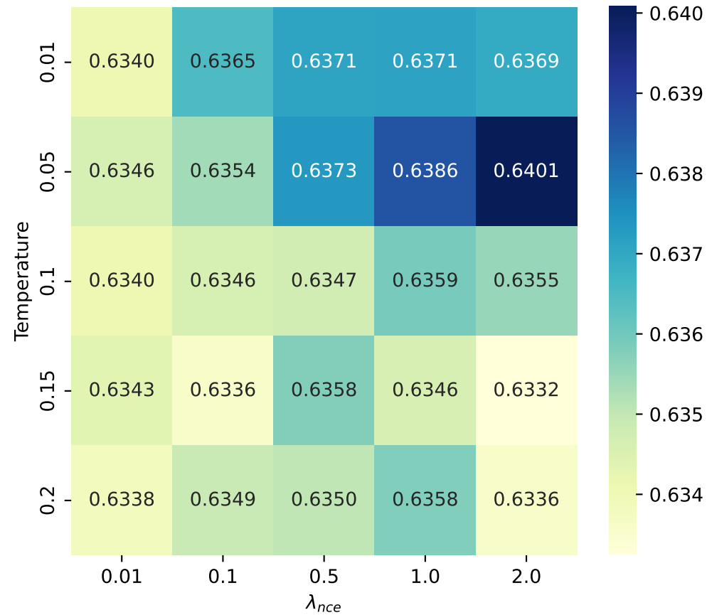
Dataset: AWM
