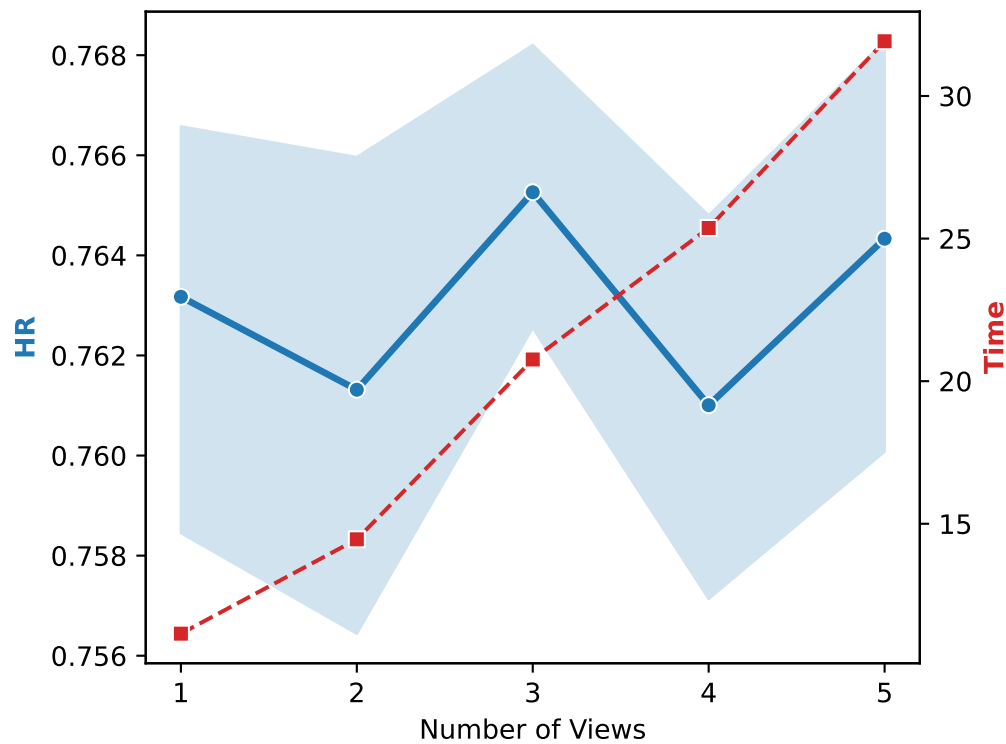
Dataset: AWM
