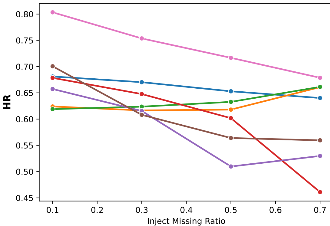
Dataset: HIP
