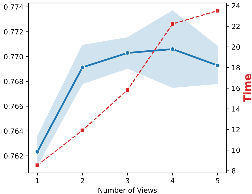
Dataset: AWM
