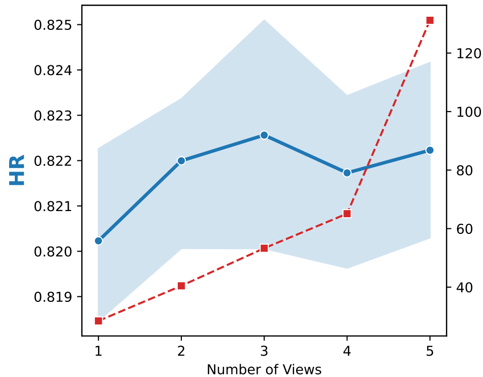
Dataset: HIP
