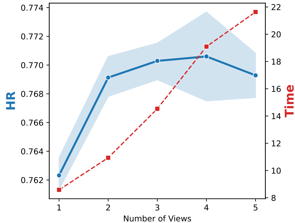
Dataset: AWM
