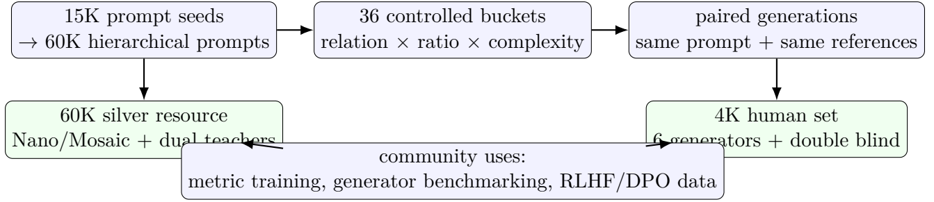
Figure 1: BindBench overview: hierarchical prompts, controlled pairs, a silver training resource, and a broader human evaluation layer.
