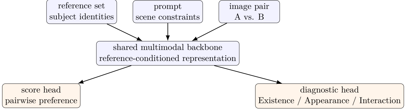
Figure 2: AnchorScore architecture: references, prompt, and paired generations are fused by a shared backbone, then decoded into ranking and diagnostic outputs.
