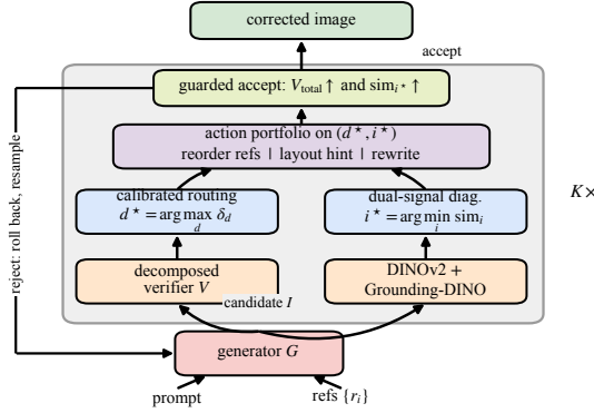
Figure 2: MIDC. The grey block runs for K correction steps. A candidate from the black-box generator is scored twice: the decomposed verifier V gives per-facet scores, and detection-aware DINOv2 gives per-subject identity. Calibrated routing picks the facet with the largest standardized deficit d^* , dual-signal diagnosis picks the weakest subject i^* , and the portfolio acts on that pair; a revision is kept only if the verifier total and \text{sim}_{i^*} both improve, else it is rolled back and resampled. On hard_058139 this routes to interaction ( \delta = +0.69 , over +0.54 and -1.08 ) and to s_d (undetected, \text{sim} = -1 ); step 1 is rejected (total -0.63 \rightarrow -0.77 ), step 2 accepted (total -0.35 , all four subjects recovered, SCR 0.00).
