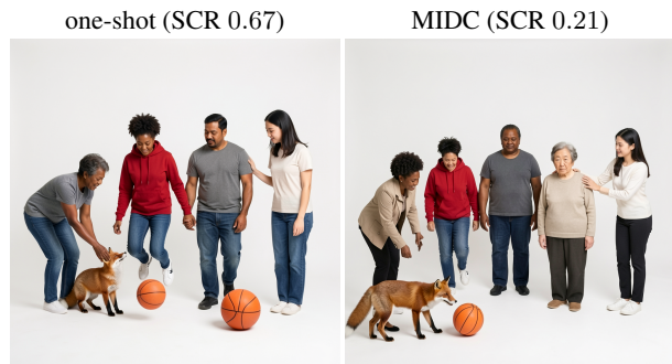
Figure 1: Interaction-induced identity collapse on an 8-entity FLUX.2-klein-9B task. One-shot generation drops 3 of 8 subjects and merges hands at contact (left, SCR 0.67); MIDC’s calibrated routing on the decomposed verifier retains more subjects with cleaner interactions (right, SCR 0.21). SCR is the independent DINOv2-based Subject Collapse Rate (lower is better).
