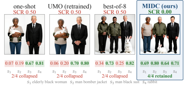
Figure 1: Interaction-induced identity collapse and correction, OmniGen2 hard 4-entity task hard_046947 , seed 0; all four panels share the seed, so they differ only in method. Cells under each image are the per-subject DINOv2 similarities that SCR thresholds at 0.5; red cells are collapsed subjects, so SCR is the fraction of red. One-shot and the retrained SOTA (UMO) fail identically: the bomber jacket bleeds onto the elderly woman and its wearer is dropped ( s_1=0.07/0.06 , s_2=0.19/0.20 ). Best-of-8 recovers him but loses the black-suit man ( s_3=0.25 ). Only MIDC clears all four. The task is one of 60 of 250 hard 4-entity tasks where MIDC is no worse than every baseline on every seed, and is not the largest-margin one (3-seed SCR means 0.58/0.58/0.50/0.33).
