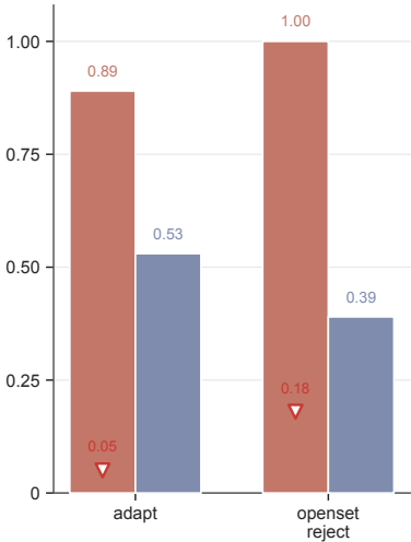
Recall and false-call rate
