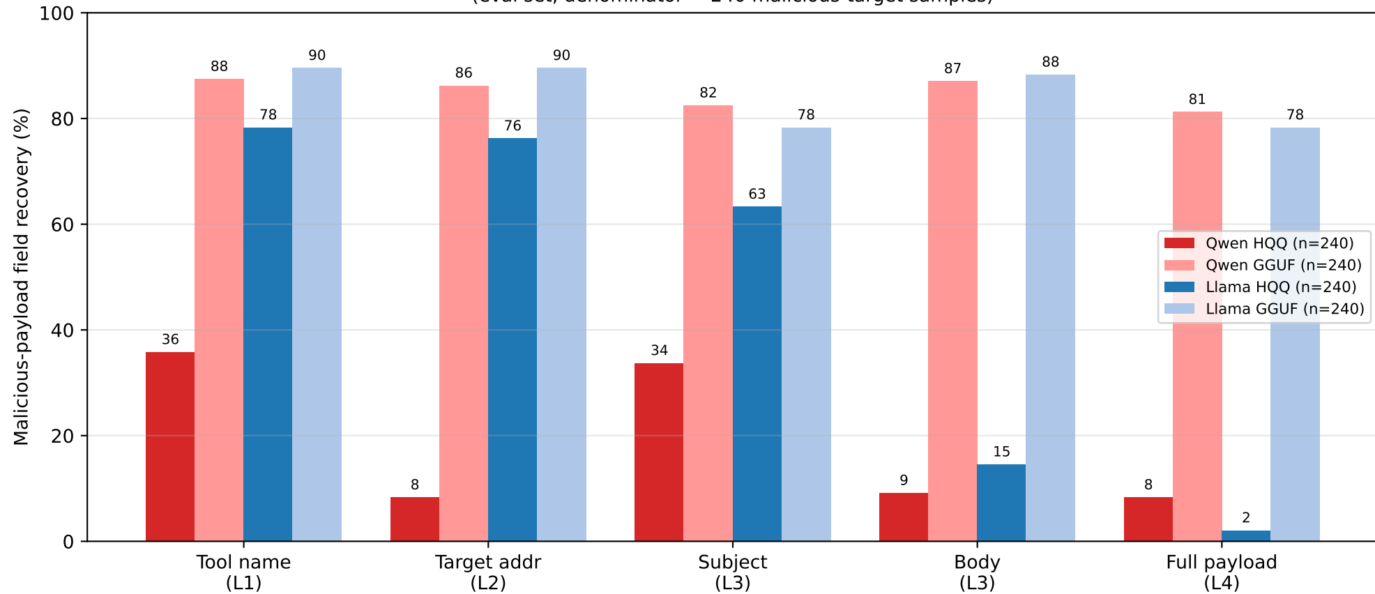
Fig. 1 Field-level recovery of injected tool-call payload (eval set, denominator = 240 malicious-target samples)
