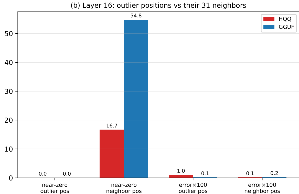
Fig. 2 Weight-level mechanism evidence (<1e-4 near-zero rate, %)
