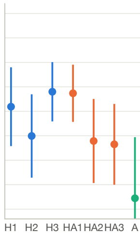
Felt genuine
