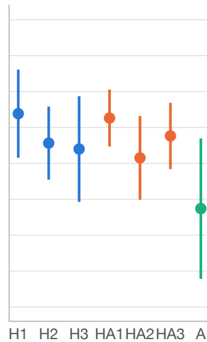
Controller warm
