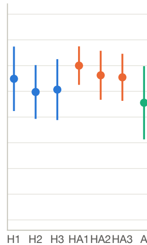
Controller competent
