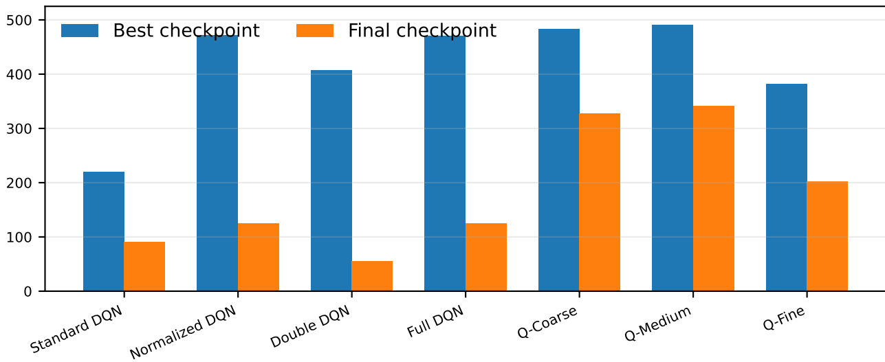
Mean episode length
